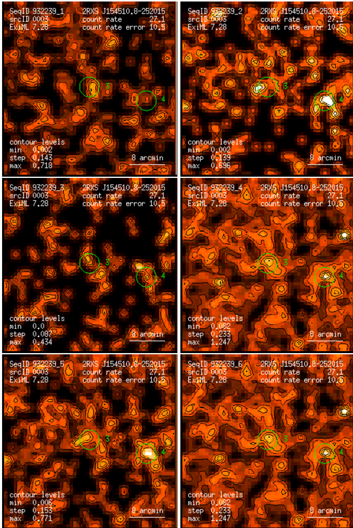
Figure 3: RASS 932239: detection 0003: band rate images, Gaussian filter: (1) PSPC channels 11 – 41, (2) 52 – 90, (3) 91 – 201, (4) 11 – 235, (5) 52 – 201, (6) 11 – 201. Broad band rates in counts/ks. Band rate contour levels in counts/ks/arcmin 2 .
