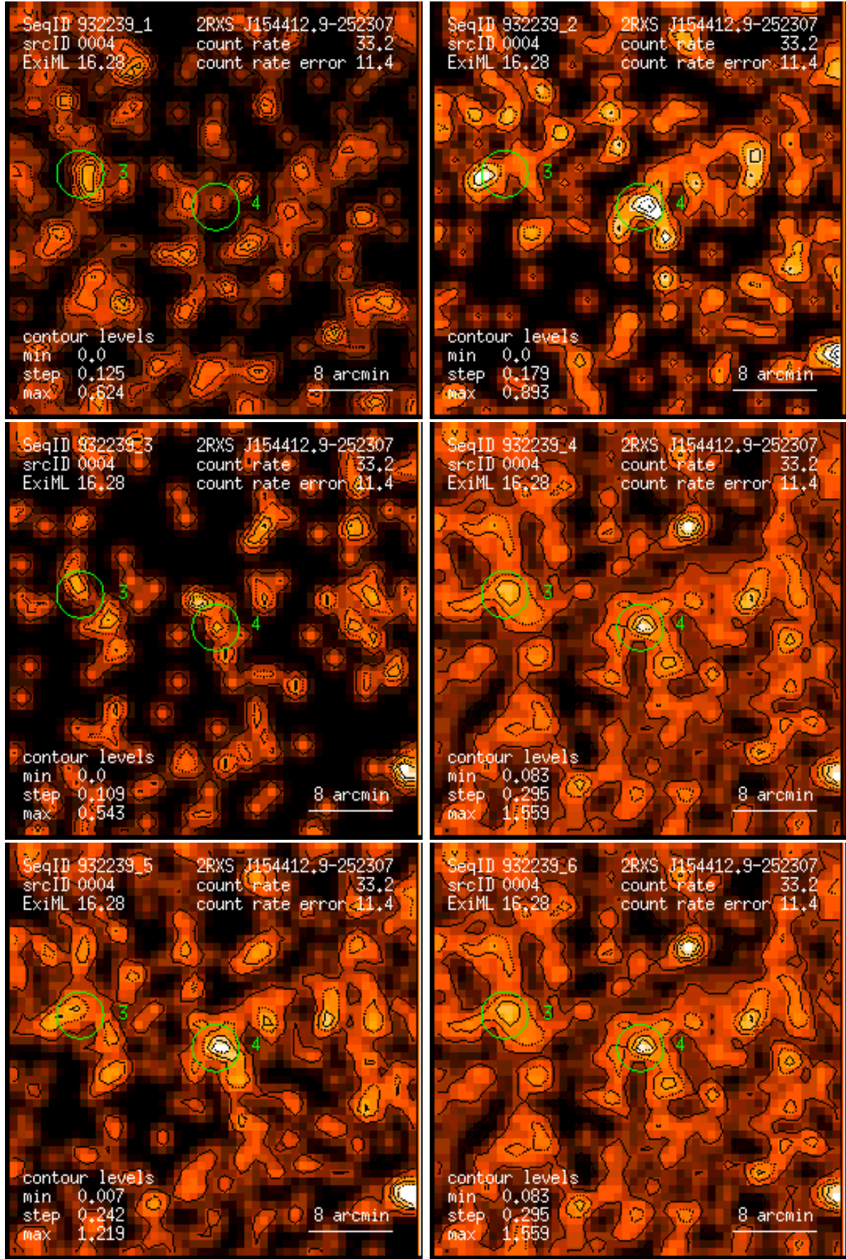
Figure 4: RASS 932239: detection 0004: band rate images, Gaussian filter: (1) PSPC channels 11 – 41, (2) 52 – 90, (3) 91 – 201, (4) 11 – 235, (5) 52 – 201, (6) 11 – 201. Broad band rates in counts/ks. Band rate contour levels in counts/ks/arcmin 2 .
