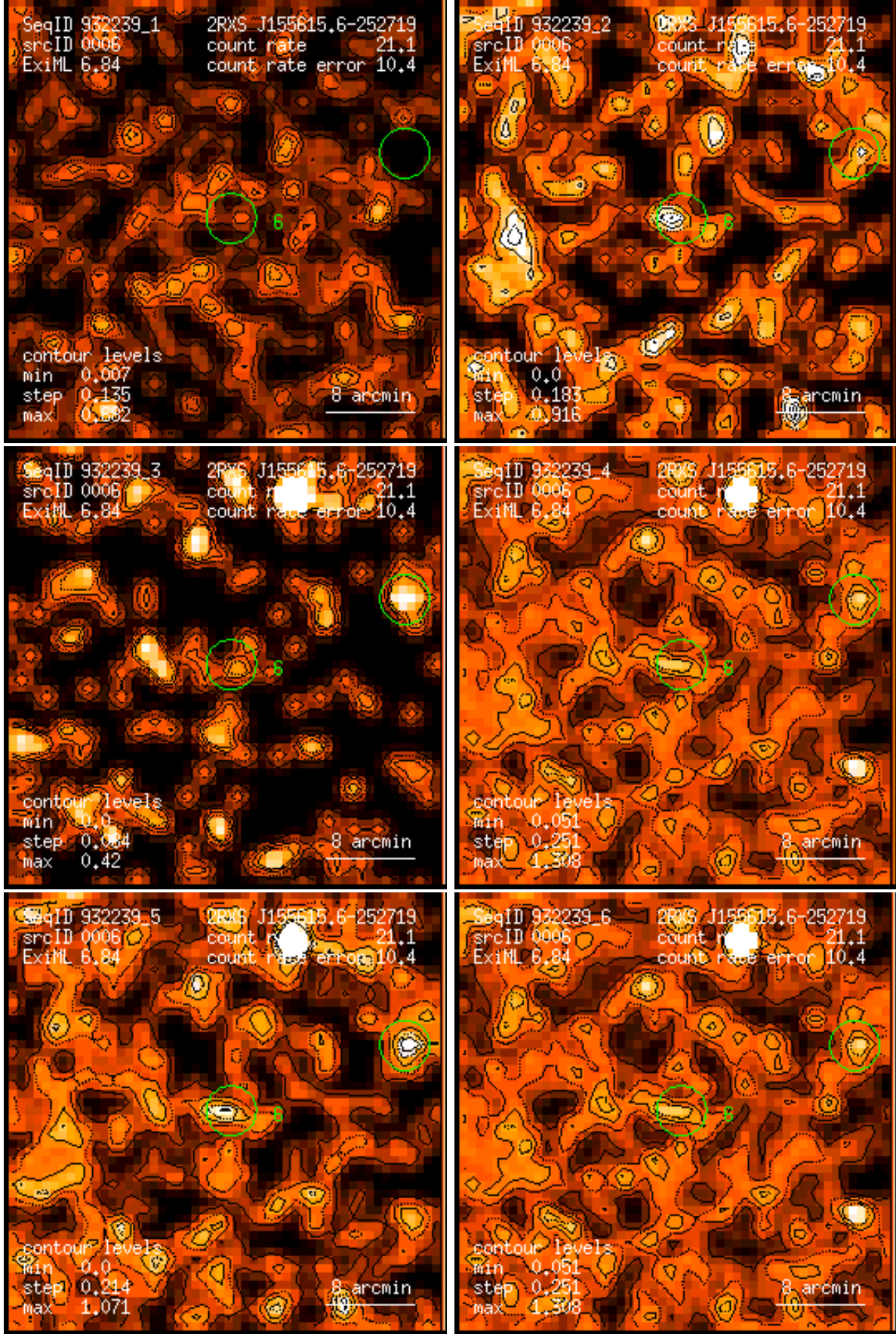
Figure 6: RASS 932239: detection 0006: band rate images, Gaussian filter: (1) PSPC channels 11 – 41, (2) 52 – 90, (3) 91 – 201, (4) 11 – 235, (5) 52 – 201, (6) 11 – 201. Broad band rates in counts/ks. Band rate contour levels in counts/ks/arcmin 2 .
