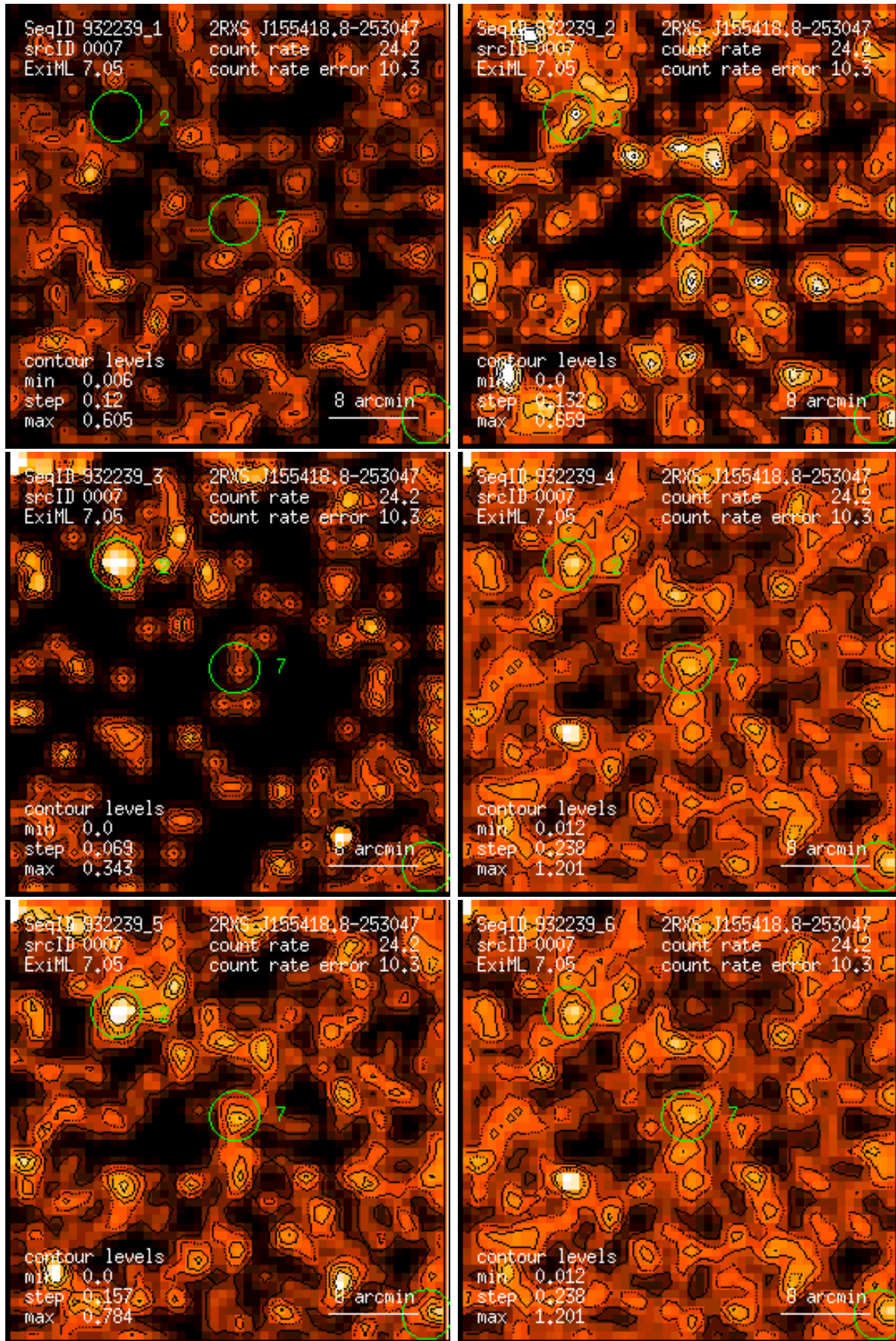
Figure 7: RASS 932239: detection 0007: band rate images, Gaussian filter: (1) PSPC channels 11 – 41, (2) 52 – 90, (3) 91 – 201, (4) 11 – 235, (5) 52 – 201, (6) 11 – 201. Broad band rates in counts/ks. Band rate contour levels in counts/ks/arcmin 2 .
