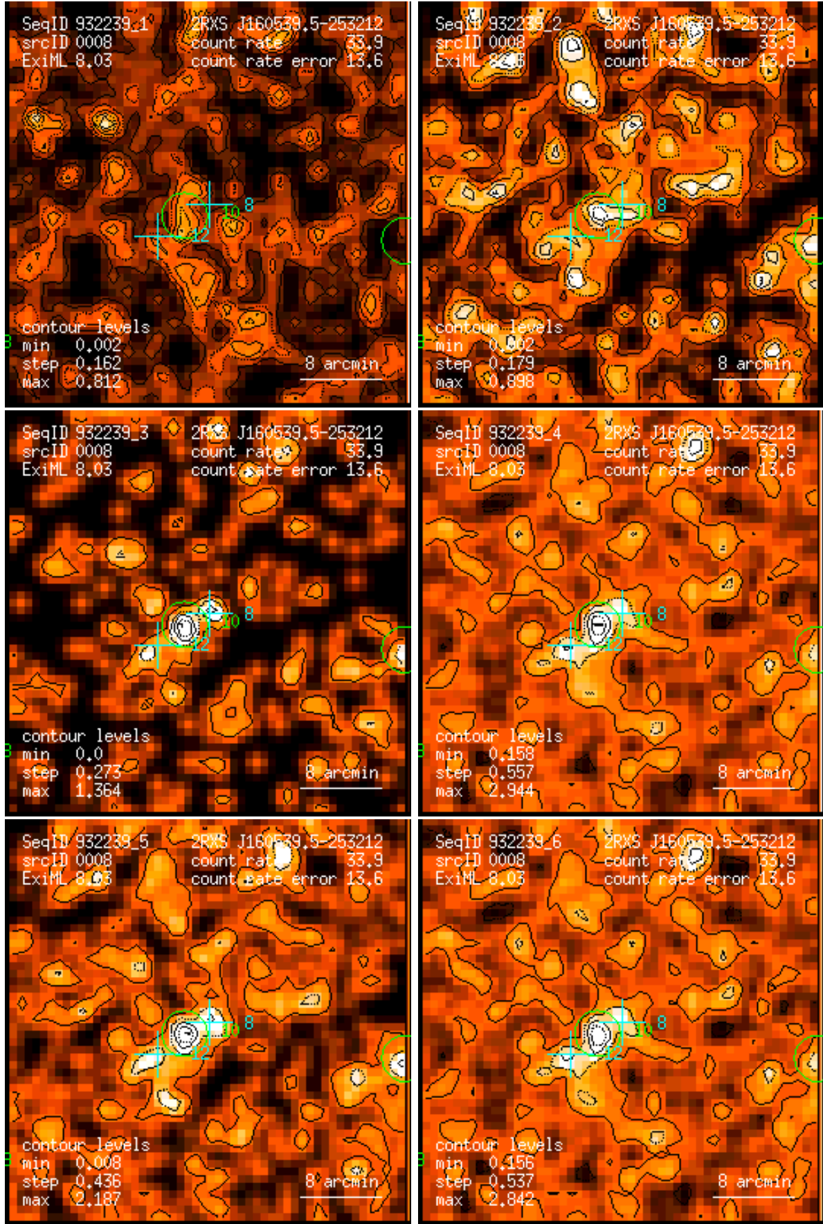
Figure 8: RASS 932239: detection 0008: band rate images, Gaussian filter: (1) PSPC channels 11 – 41, (2) 52 – 90, (3) 91 – 201, (4) 11 – 235, (5) 52 – 201, (6) 11 – 201. Broad band rates in counts/ks. Band rate contour levels in counts/ks/arcmin 2 .
