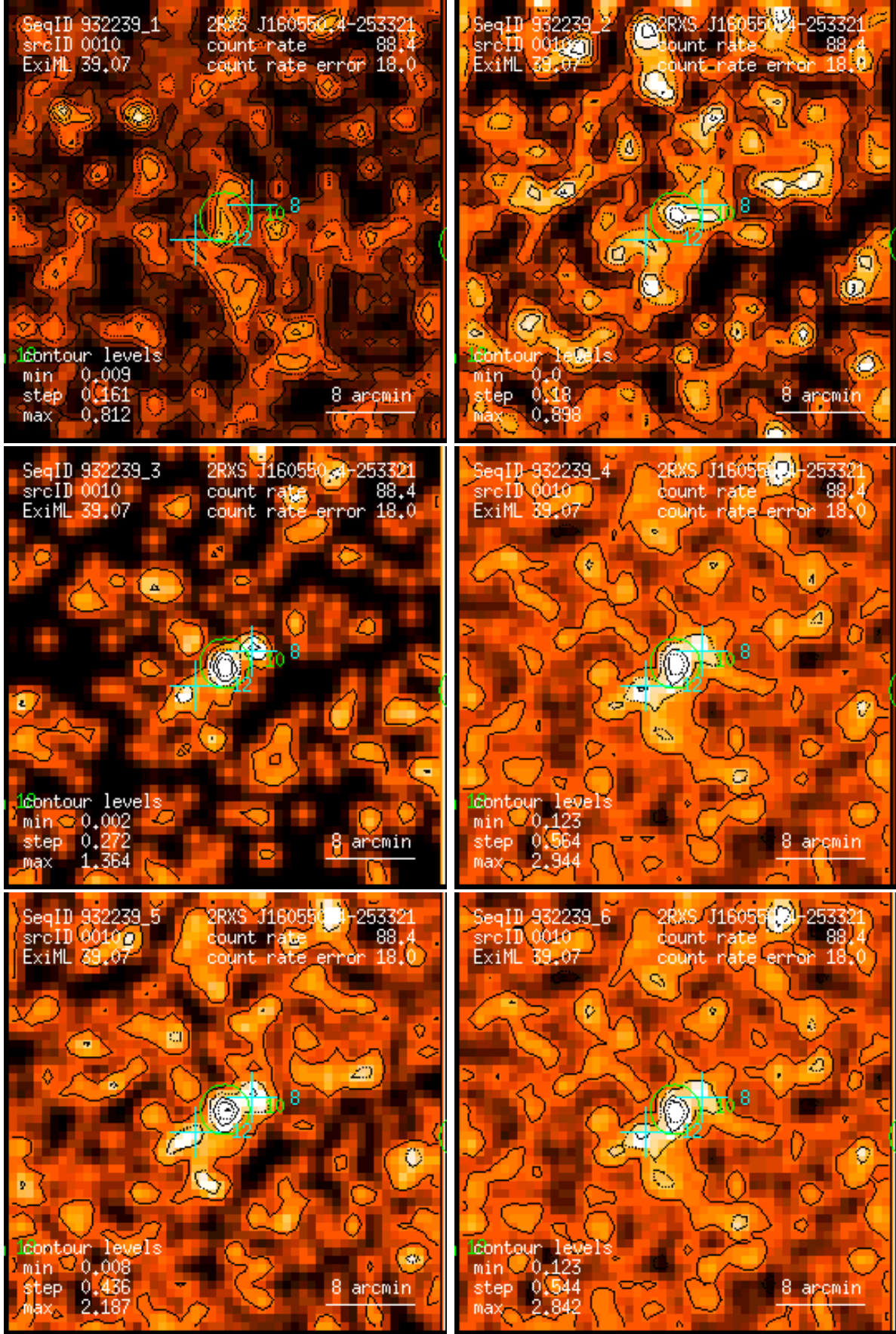
Figure 10: RASS 932239: detection 0010: band rate images, Gaussian filter: (1) PSPC channels 11 – 41, (2) 52 – 90, (3) 91 – 201, (4) 11 – 235, (5) 52 – 201, (6) 11 – 201. Broad band rates in counts/ks. Band rate contour levels in counts/ks/arcmin 2 .
