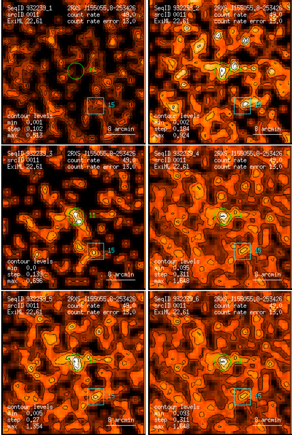
Figure 11: RASS 932239: detection 0011: band rate images, Gaussian filter: (1) PSPC channels 11 – 41, (2) 52 – 90, (3) 91 – 201, (4) 11 – 235, (5) 52 – 201, (6) 11 – 201. Broad band rates in counts/ks. Band rate contour levels in counts/ks/arcmin 2 .
