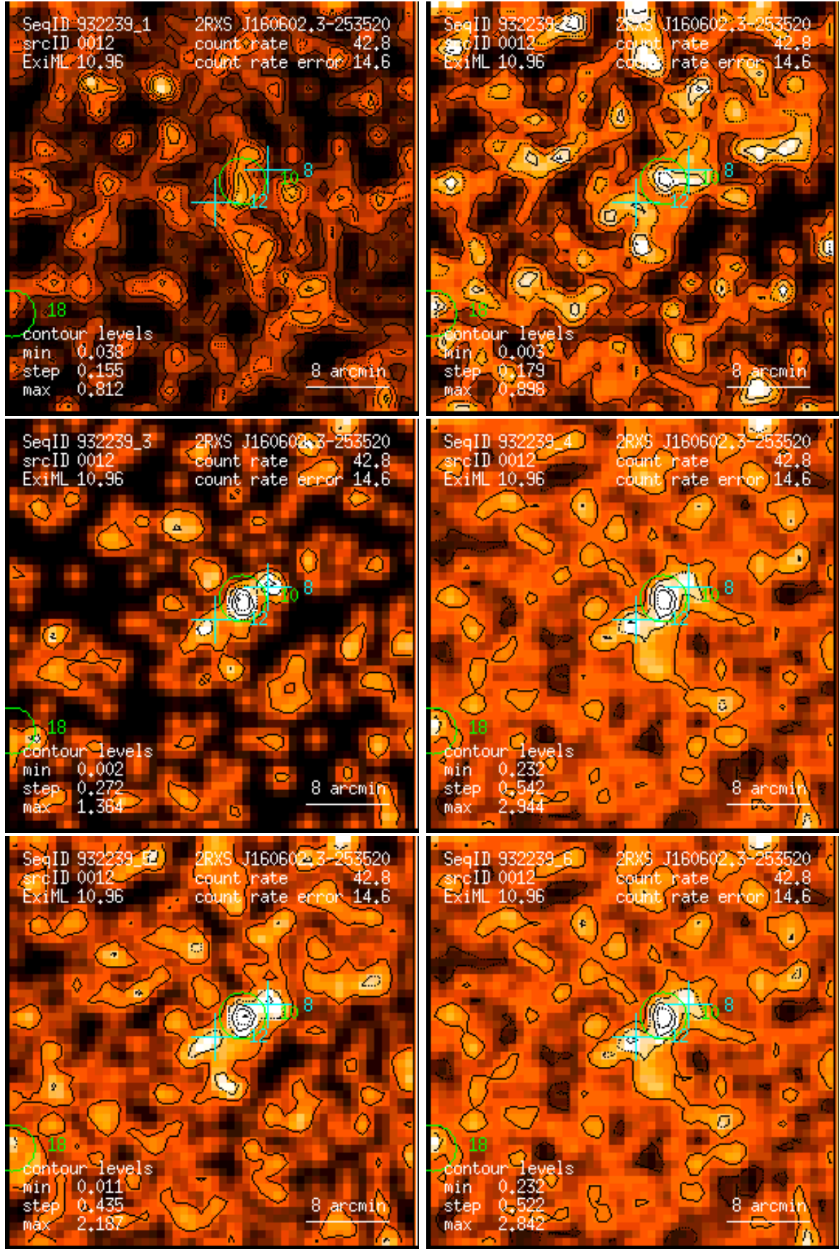
Figure 12: RASS 932239: detection 0012: band rate images, Gaussian filter: (1) PSPC channels 11 – 41, (2) 52 – 90, (3) 91 – 201, (4) 11 – 235, (5) 52 – 201, (6) 11 – 201. Broad band rates in counts/ks. Band rate contour levels in counts/ks/arcmin 2 .
