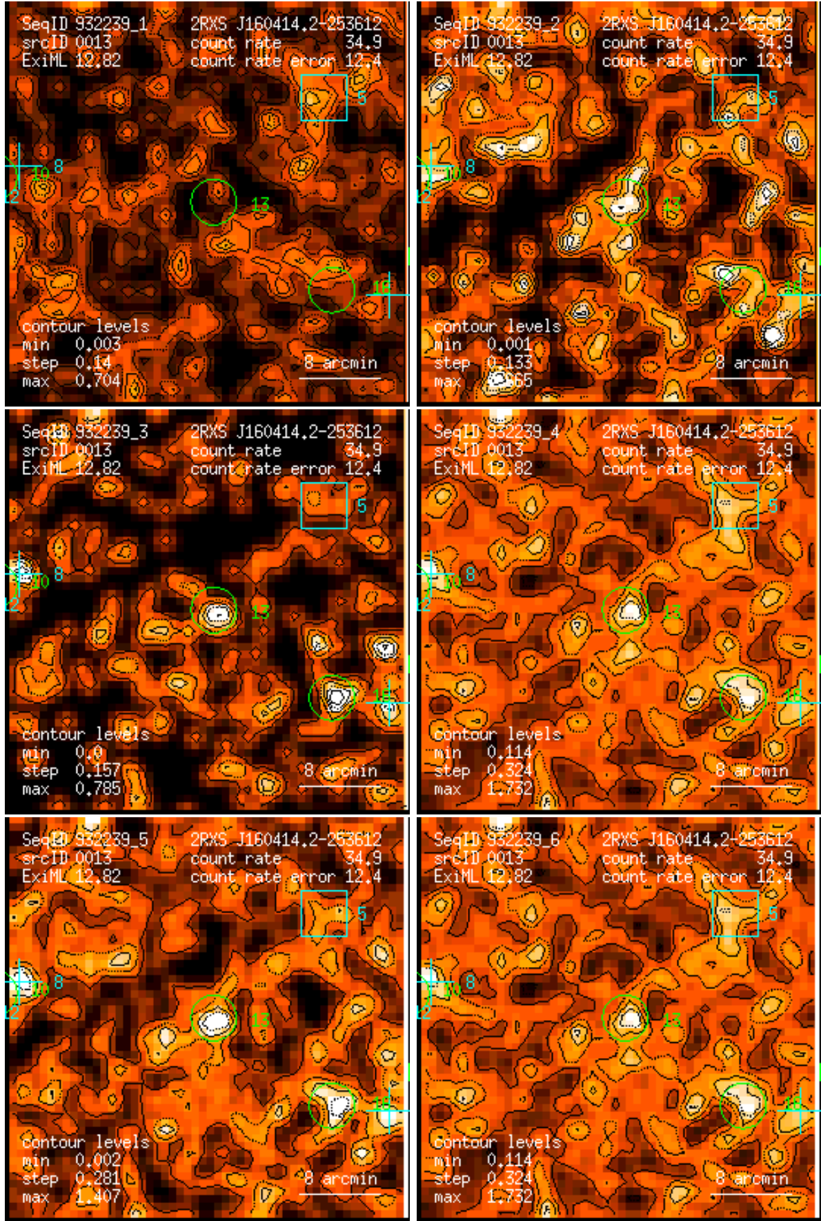
Figure 13: RASS 932239: detection 0013: band rate images, Gaussian filter: (1) PSPC channels 11 – 41, (2) 52 – 90, (3) 91 – 201, (4) 11 – 235, (5) 52 – 201, (6) 11 – 201. Broad band rates in counts/ks. Band rate contour levels in counts/ks/arcmin 2 .
