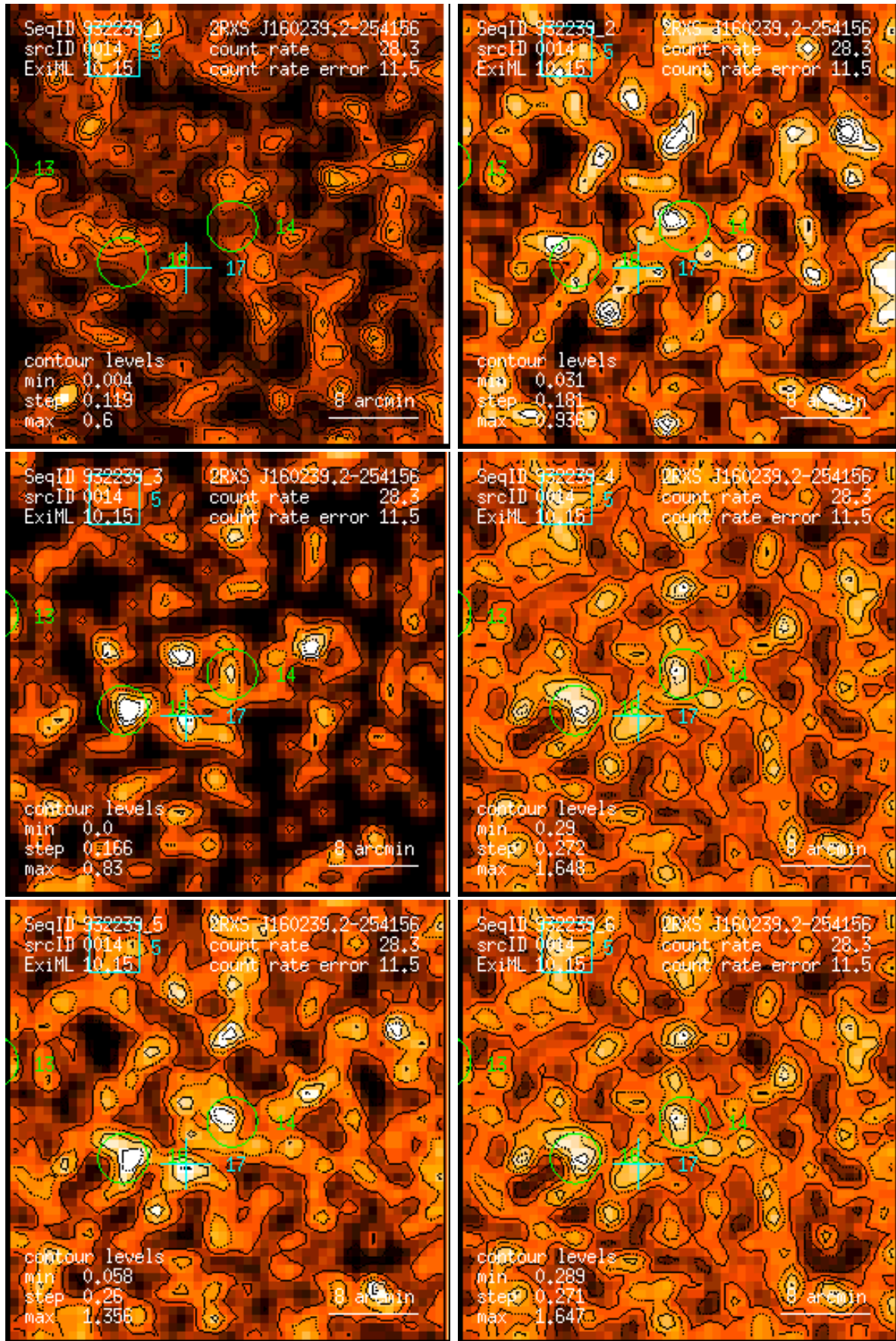
Figure 14: RASS 932239: detection 0014: band rate images, Gaussian filter: (1) PSPC channels 11 – 41, (2) 52 – 90, (3) 91 – 201, (4) 11 – 235, (5) 52 – 201, (6) 11 – 201. Broad band rates in counts/ks. Band rate contour levels in counts/ks/arcmin 2 .
