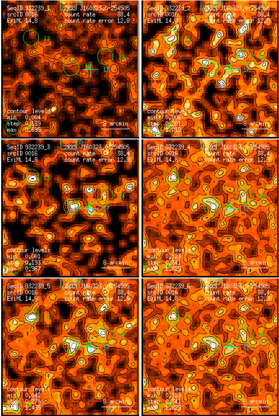
Figure 16: RASS 932239: detection 0016: band rate images, Gaussian filter: (1) PSPC channels 11 – 41, (2) 52 – 90, (3) 91 – 201, (4) 11 – 235, (5) 52 – 201, (6) 11 – 201. Broad band rates in counts/ks. Band rate contour levels in counts/ks/arcmin 2 .
