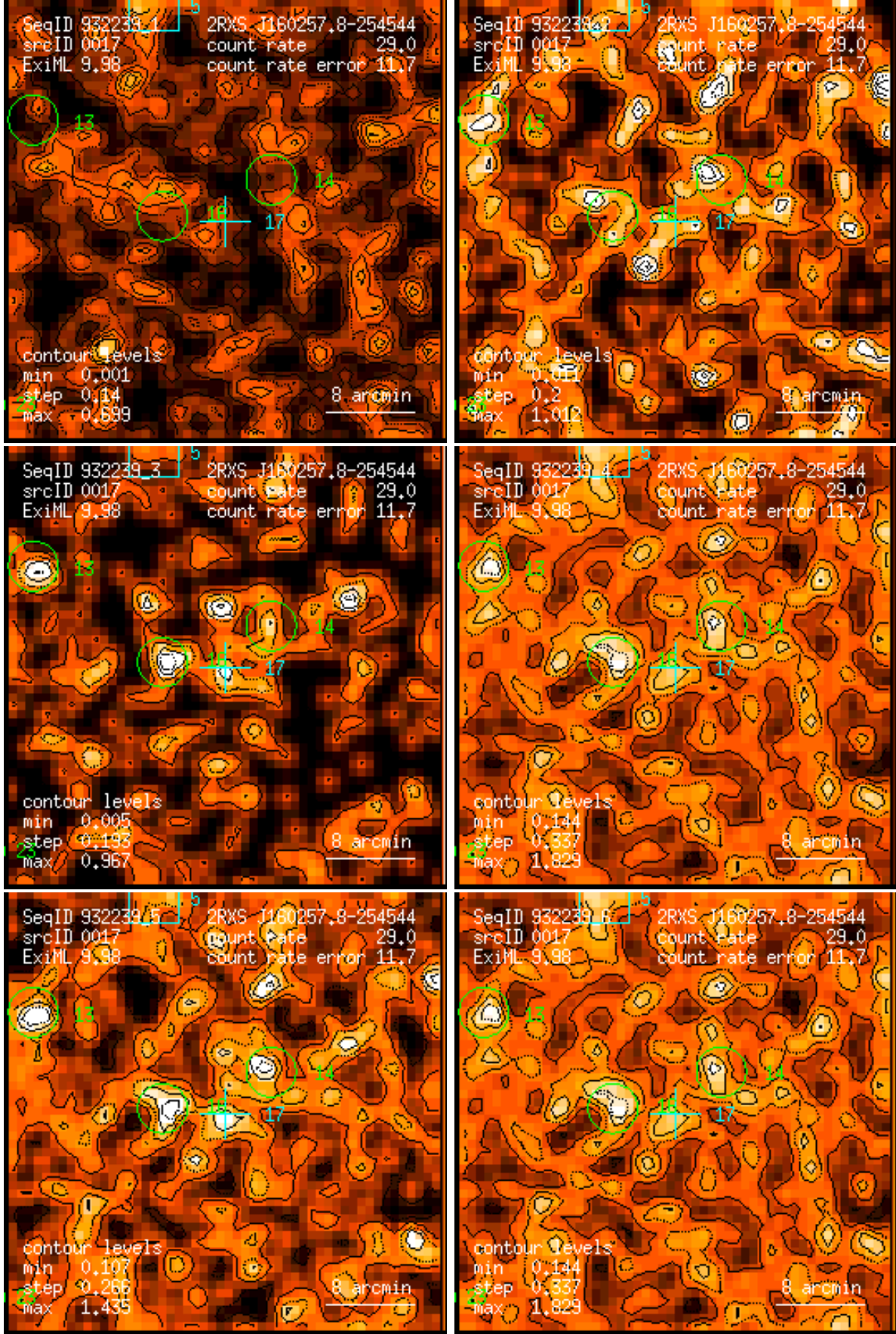
Figure 17: RASS 932239: detection 0017: band rate images, Gaussian filter: (1) PSPC channels 11 – 41, (2) 52 – 90, (3) 91 – 201, (4) 11 – 235, (5) 52 – 201, (6) 11 – 201. Broad band rates in counts/ks. Band rate contour levels in counts/ks/arcmin 2 .
