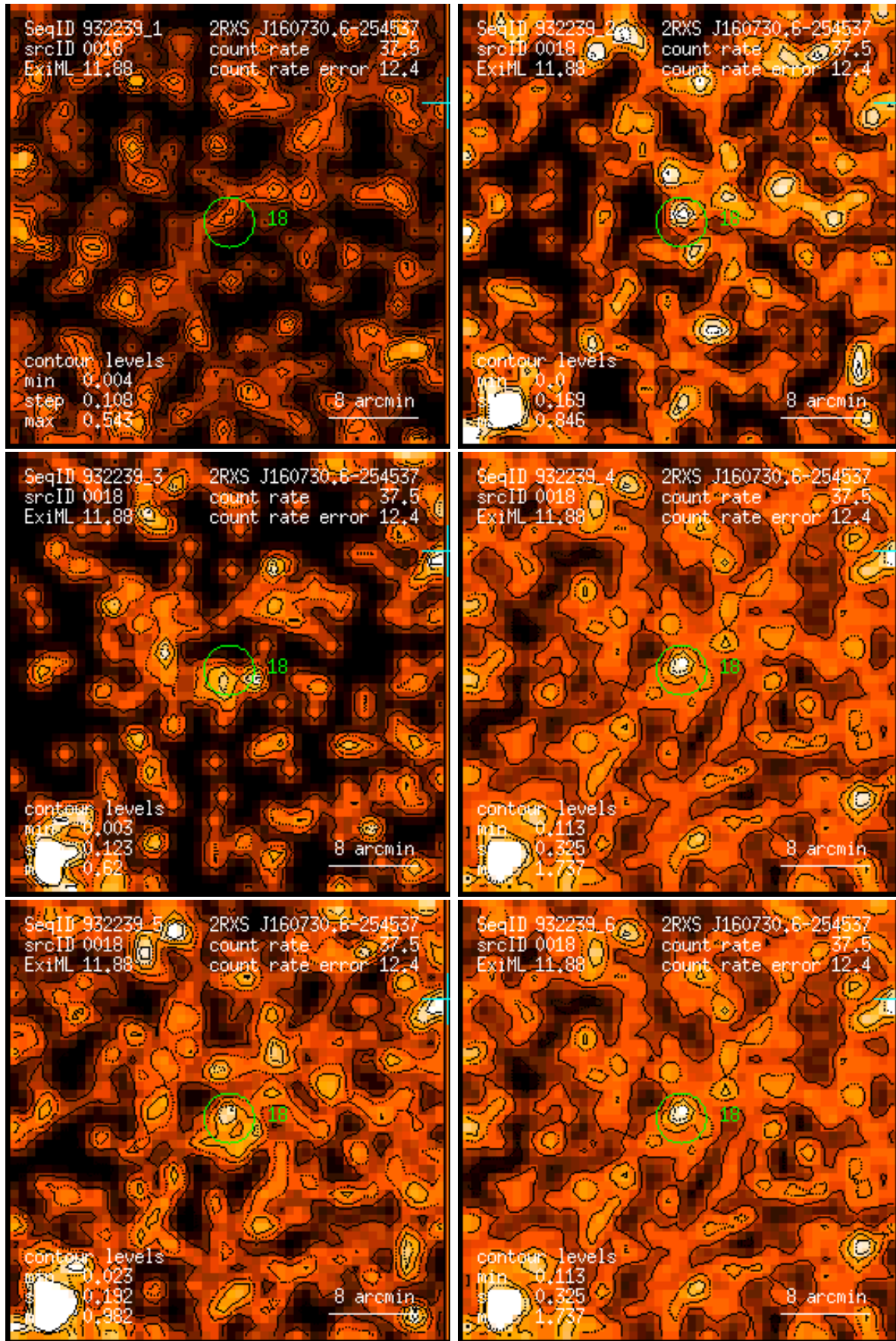
Figure 18: RASS 932239: detection 0018: band rate images, Gaussian filter: (1) PSPC channels 11 – 41, (2) 52 – 90, (3) 91 – 201, (4) 11 – 235, (5) 52 – 201, (6) 11 – 201. Broad band rates in counts/ks. Band rate contour levels in counts/ks/arcmin 2 .
