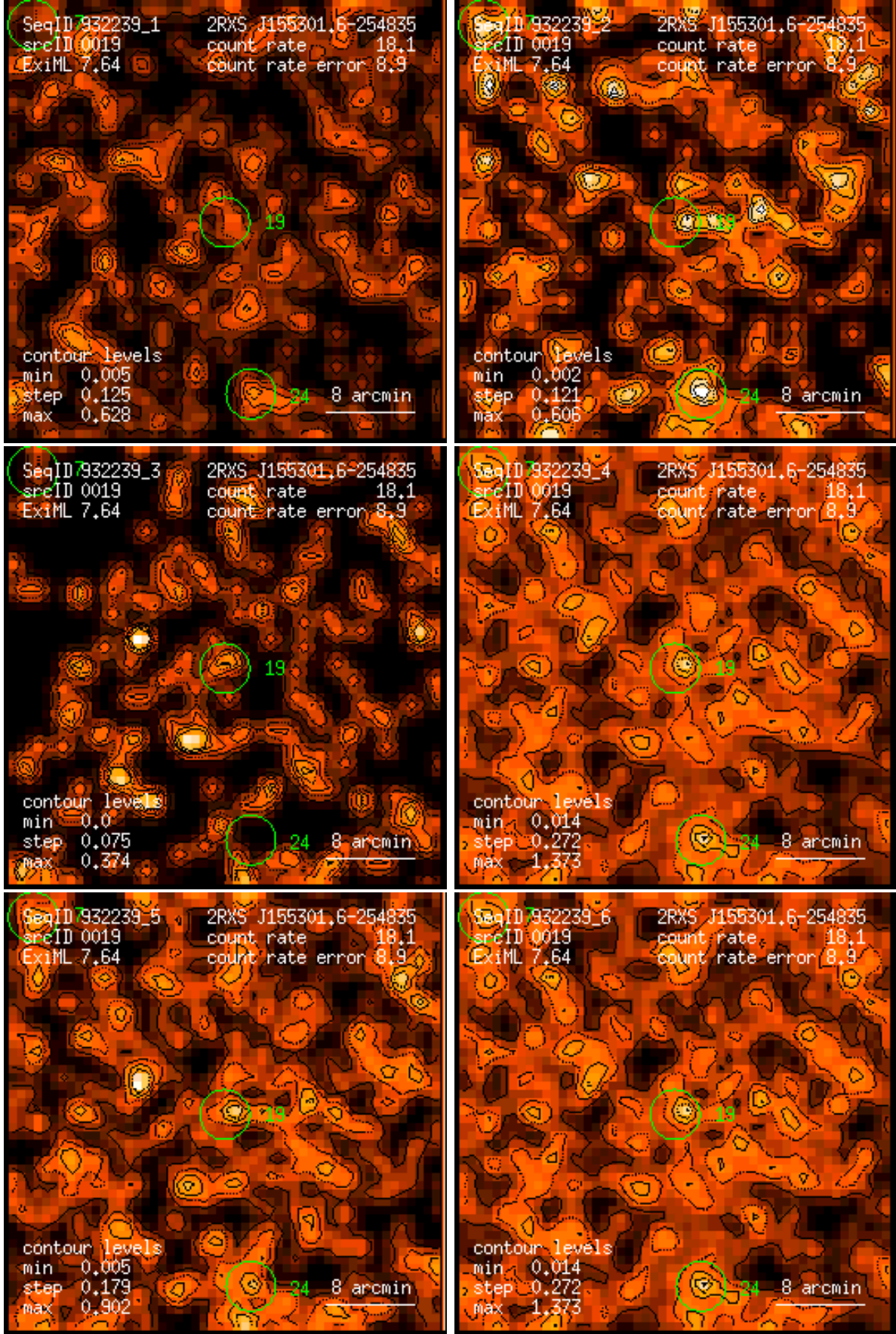
Figure 19: RASS 932239: detection 0019: band rate images, Gaussian filter: (1) PSPC channels 11 – 41, (2) 52 – 90, (3) 91 – 201, (4) 11 – 235, (5) 52 – 201, (6) 11 – 201. Broad band rates in counts/ks. Band rate contour levels in counts/ks/arcmin 2 .
