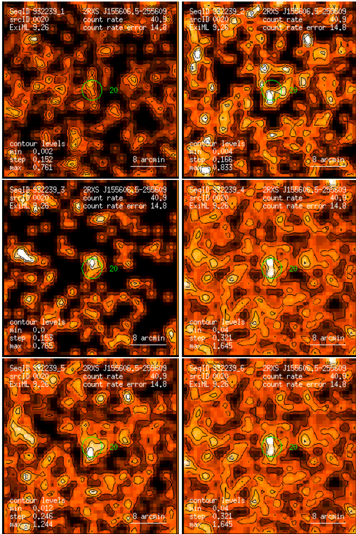
Figure 20: RASS 932239: detection 0020: band rate images, Gaussian filter: (1) PSPC channels 11 – 41, (2) 52 – 90, (3) 91 – 201, (4) 11 – 235, (5) 52 – 201, (6) 11 – 201. Broad band rates in counts/ks. Band rate contour levels in counts/ks/arcmin 2 .
