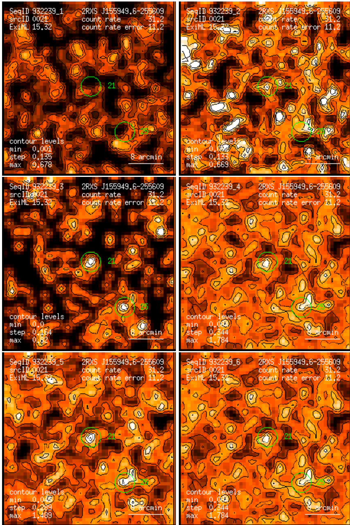
Figure 21: RASS 932239: detection 0021: band rate images, Gaussian filter: (1) PSPC channels 11 – 41, (2) 52 – 90, (3) 91 – 201, (4) 11 – 235, (5) 52 – 201, (6) 11 – 201. Broad band rates in counts/ks. Band rate contour levels in counts/ks/arcmin 2 .
