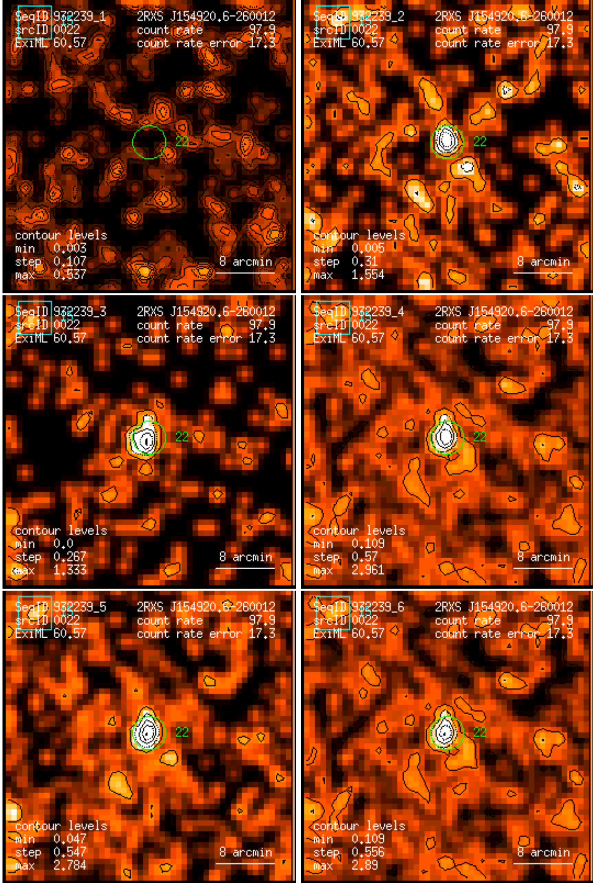
Figure 22: RASS 932239: detection 0022: band rate images, Gaussian filter: (1) PSPC channels 11 – 41, (2) 52 – 90, (3) 91 – 201, (4) 11 – 235, (5) 52 – 201, (6) 11 – 201. Broad band rates in counts/ks. Band rate contour levels in counts/ks/arcmin 2 .
