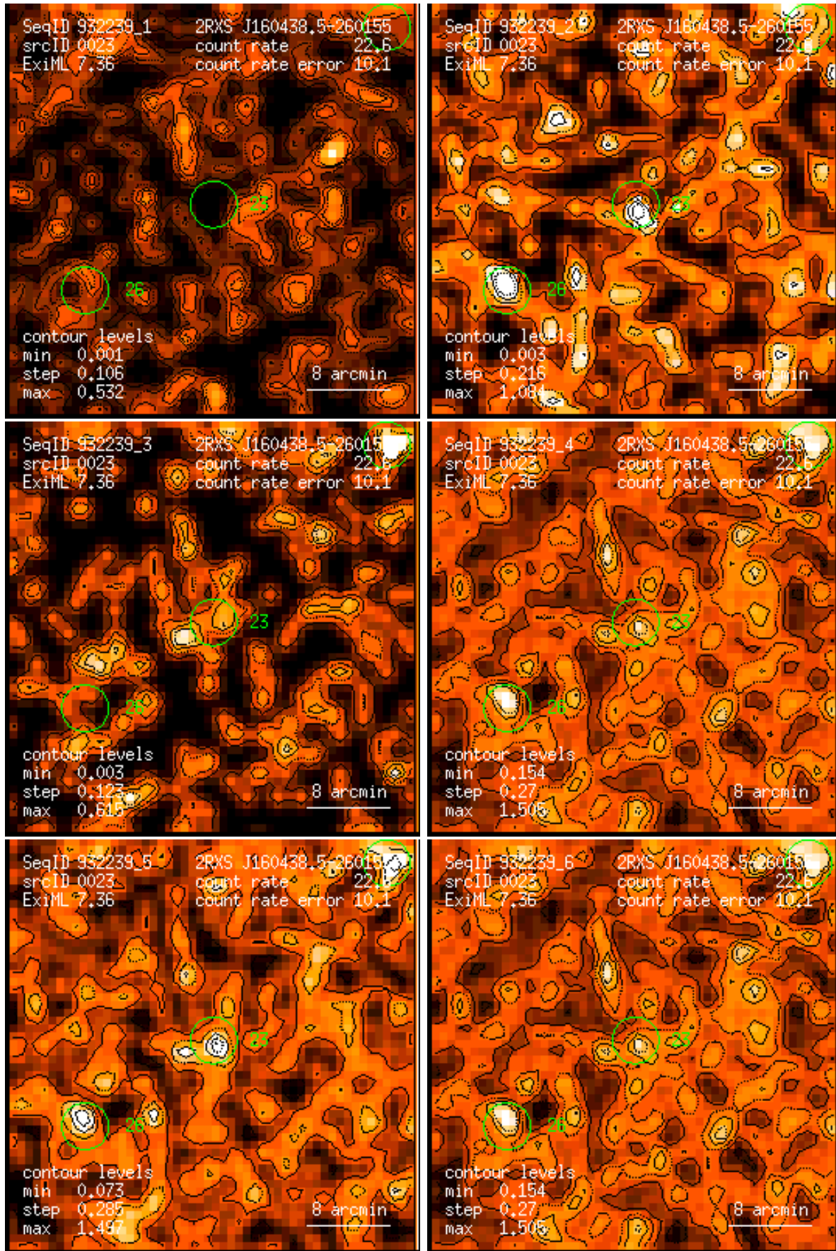
Figure 23: RASS 932239: detection 0023: band rate images, Gaussian filter: (1) PSPC channels 11 – 41, (2) 52 – 90, (3) 91 – 201, (4) 11 – 235, (5) 52 – 201, (6) 11 – 201. Broad band rates in counts/ks. Band rate contour levels in counts/ks/arcmin 2 .
