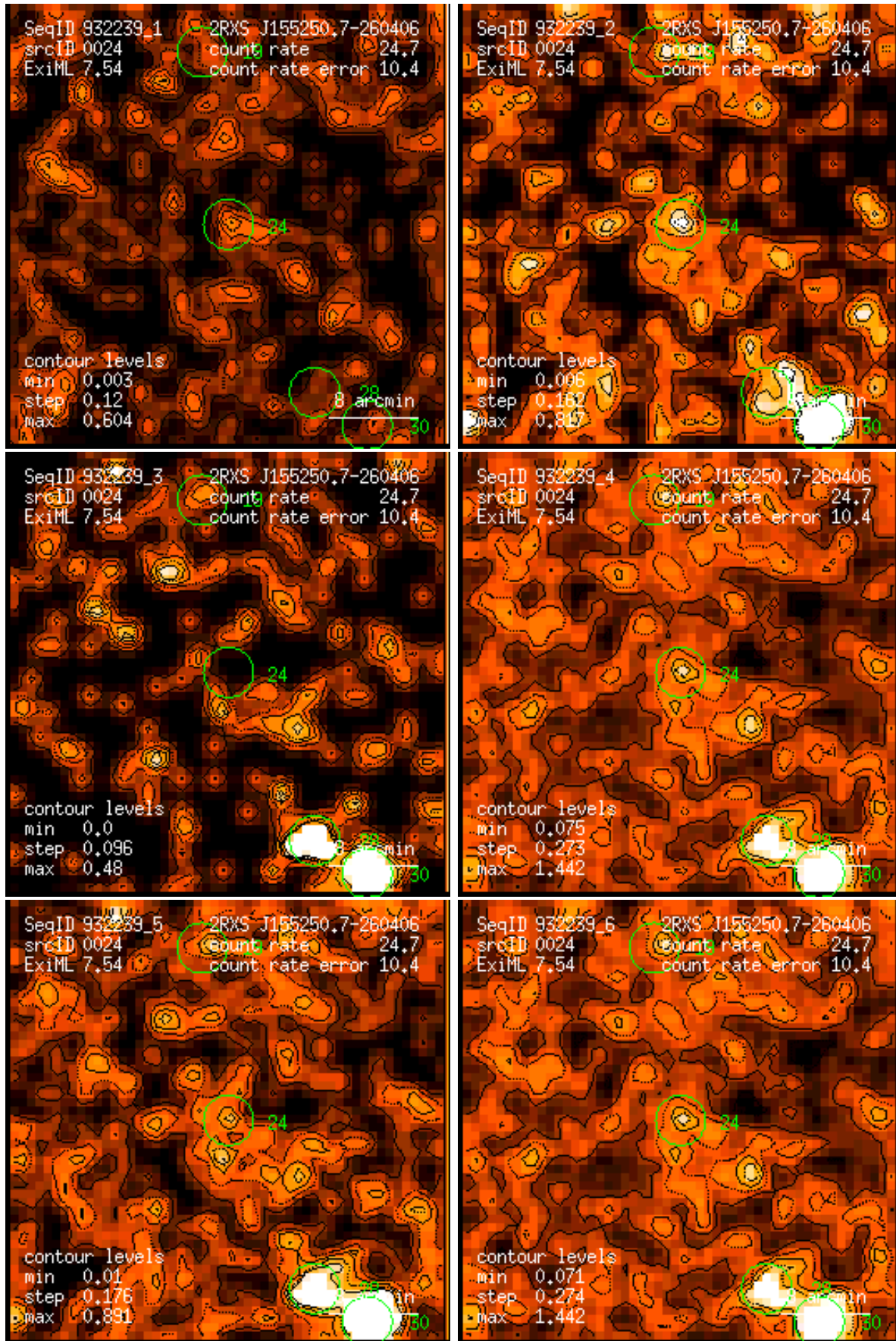
Figure 24: RASS 932239: detection 0024: band rate images, Gaussian filter: (1) PSPC channels 11 – 41, (2) 52 – 90, (3) 91 – 201, (4) 11 – 235, (5) 52 – 201, (6) 11 – 201. Broad band rates in counts/ks. Band rate contour levels in counts/ks/arcmin 2 .
