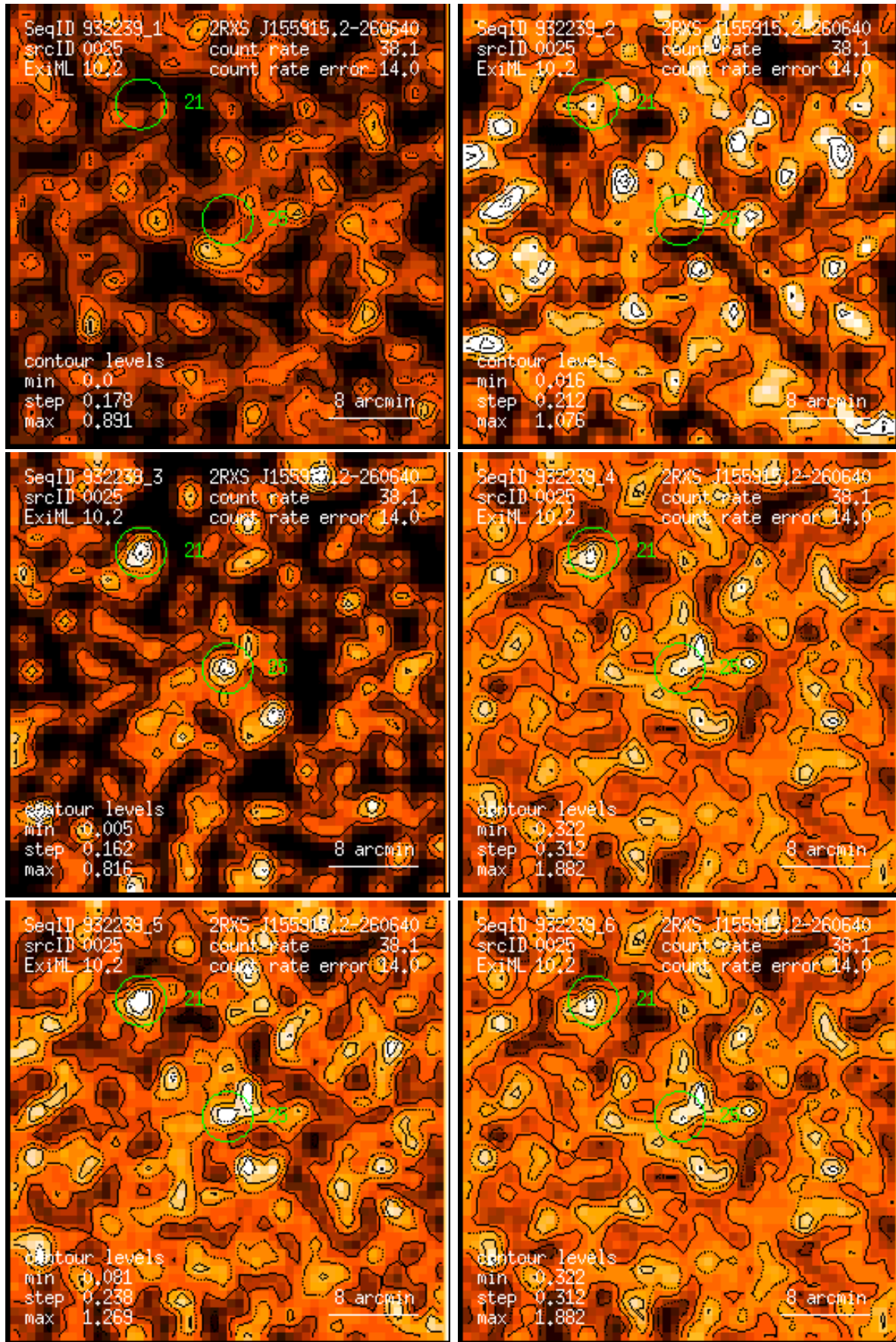
Figure 25: RASS 932239: detection 0025: band rate images, Gaussian filter: (1) PSPC channels 11 – 41, (2) 52 – 90, (3) 91 – 201, (4) 11 – 235, (5) 52 – 201, (6) 11 – 201. Broad band rates in counts/ks. Band rate contour levels in counts/ks/arcmin 2 .
