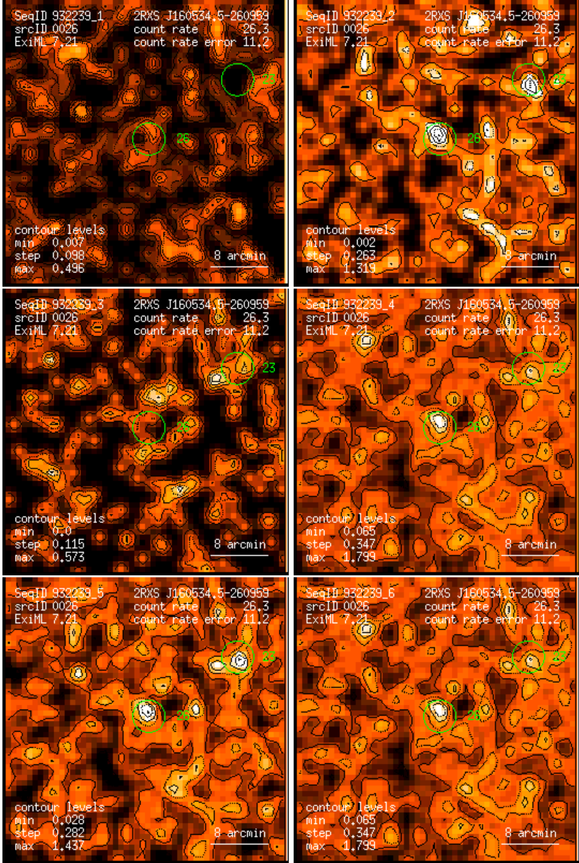
Figure 26: RASS 932239: detection 0026: band rate images, Gaussian filter: (1) PSPC channels 11 – 41, (2) 52 – 90, (3) 91 – 201, (4) 11 – 235, (5) 52 – 201, (6) 11 – 201. Broad band rates in counts/ks. Band rate contour levels in counts/ks/arcmin 2 .
