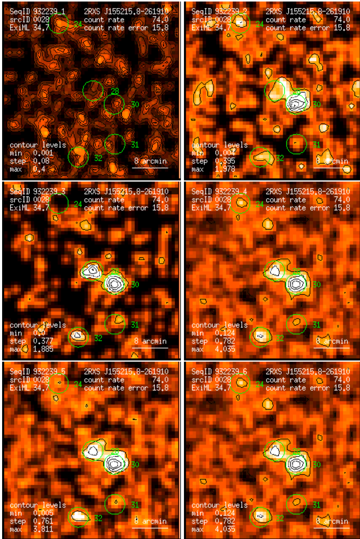
Figure 28: RASS 932239: detection 0028: band rate images, Gaussian filter: (1) PSPC channels 11 – 41, (2) 52 – 90, (3) 91 – 201, (4) 11 – 235, (5) 52 – 201, (6) 11 – 201. Broad band rates in counts/ks. Band rate contour levels in counts/ks/arcmin 2 .
