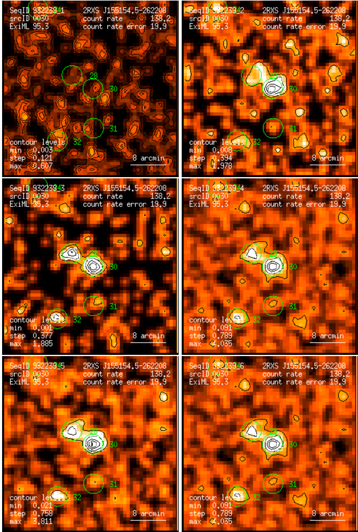
Figure 30: RASS 932239: detection 0030: band rate images, Gaussian filter: (1) PSPC channels 11 – 41, (2) 52 – 90, (3) 91 – 201, (4) 11 – 235, (5) 52 – 201, (6) 11 – 201. Broad band rates in counts/ks. Band rate contour levels in counts/ks/arcmin 2 .
