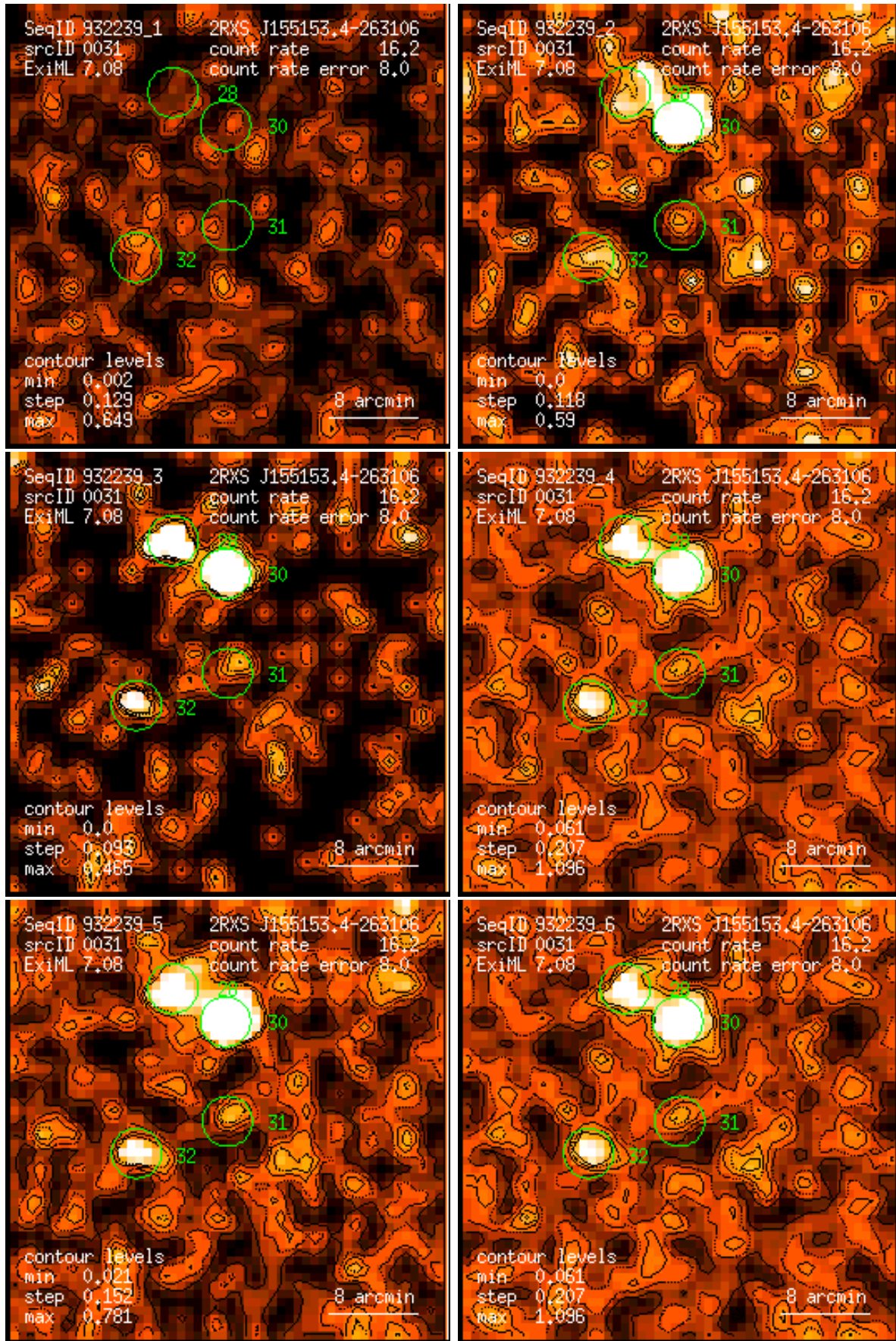
Figure 31: RASS 932239: detection 0031: band rate images, Gaussian filter: (1) PSPC channels 11 – 41, (2) 52 – 90, (3) 91 – 201, (4) 11 – 235, (5) 52 – 201, (6) 11 – 201. Broad band rates in counts/ks. Band rate contour levels in counts/ks/arcmin 2 .
