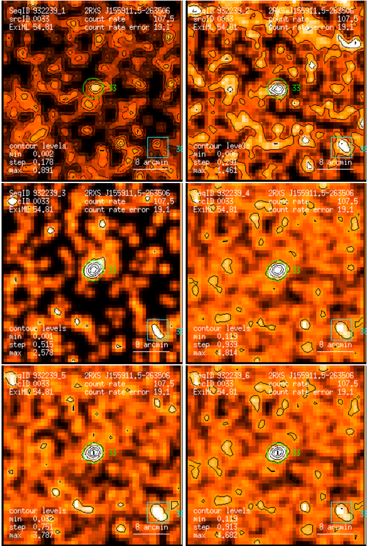
Figure 33: RASS 932239: detection 0033: band rate images, Gaussian filter: (1) PSPC channels 11 – 41, (2) 52 – 90, (3) 91 – 201, (4) 11 – 235, (5) 52 – 201, (6) 11 – 201. Broad band rates in counts/ks. Band rate contour levels in counts/ks/arcmin 2 .
