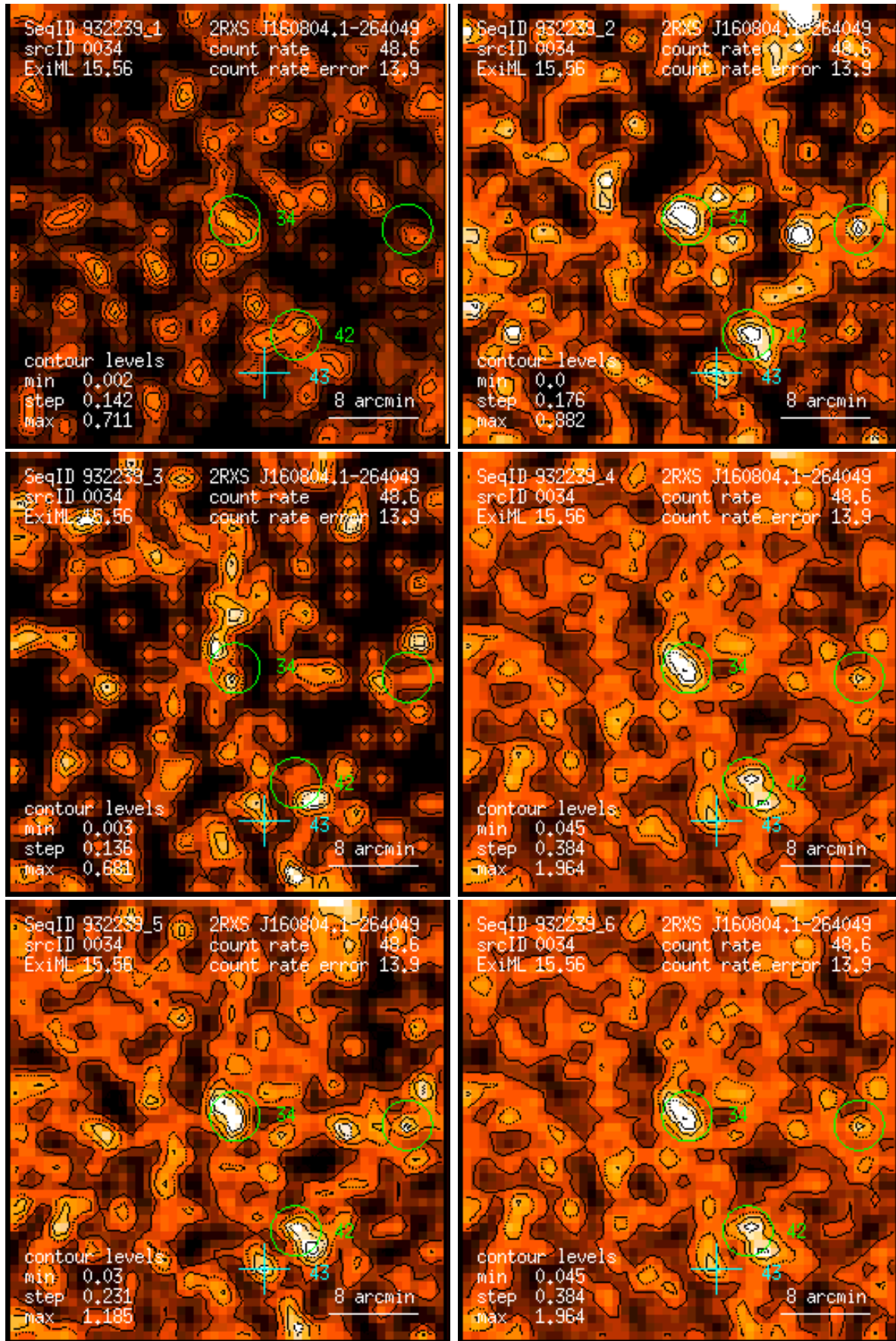
Figure 34: RASS 932239: detection 0034: band rate images, Gaussian filter: (1) PSPC channels 11 – 41, (2) 52 – 90, (3) 91 – 201, (4) 11 – 235, (5) 52 – 201, (6) 11 – 201. Broad band rates in counts/ks. Band rate contour levels in counts/ks/arcmin 2 .
