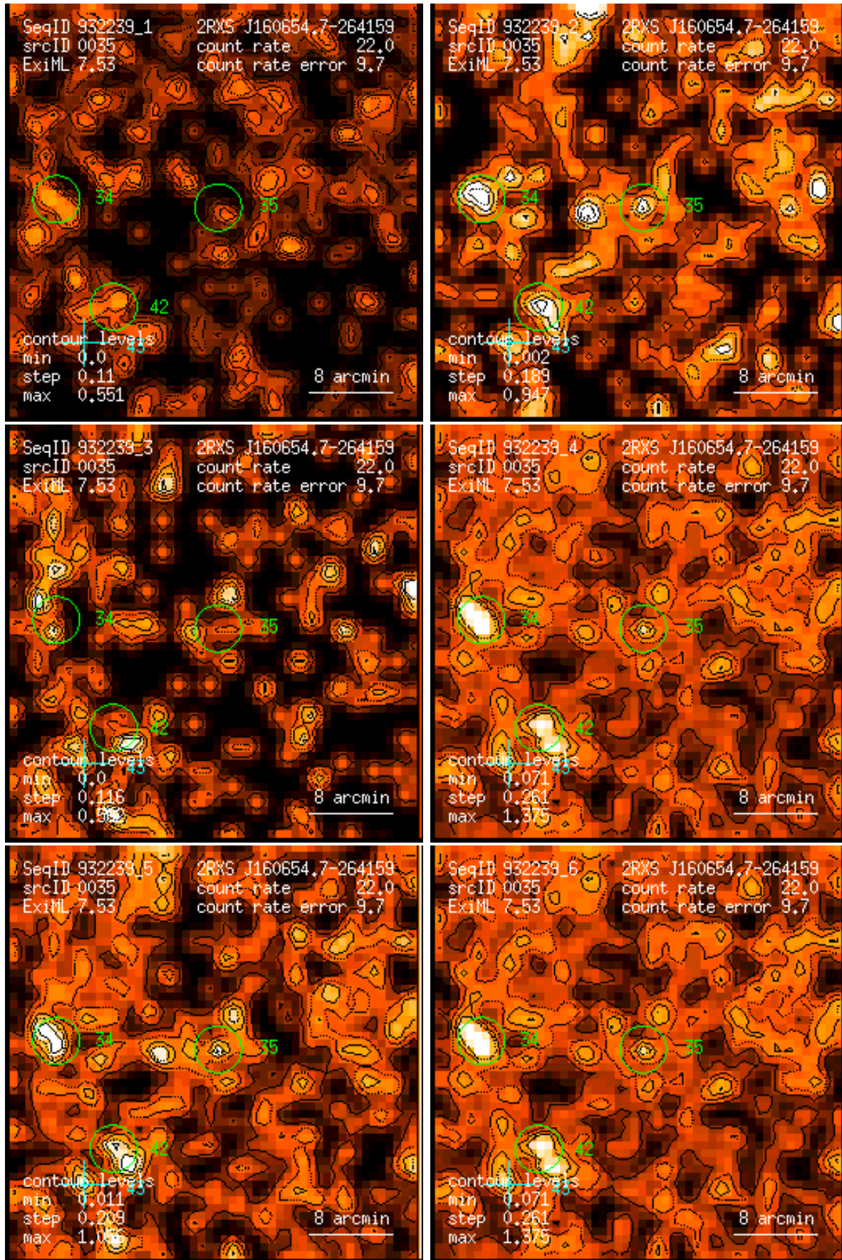
Figure 35: RASS 932239: detection 0035: band rate images, Gaussian filter: (1) PSPC channels 11 – 41, (2) 52 – 90, (3) 91 – 201, (4) 11 – 235, (5) 52 – 201, (6) 11 – 201. Broad band rates in counts/ks. Band rate contour levels in counts/ks/arcmin 2 .
