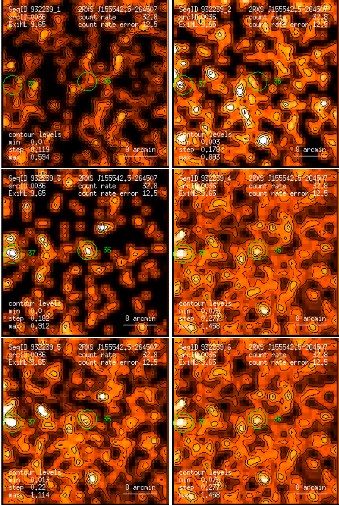
Figure 36: RASS 932239: detection 0036: band rate images, Gaussian filter: (1) PSPC channels 11 – 41, (2) 52 – 90, (3) 91 – 201, (4) 11 – 235, (5) 52 – 201, (6) 11 – 201. Broad band rates in counts/ks. Band rate contour levels in counts/ks/arcmin 2 .
