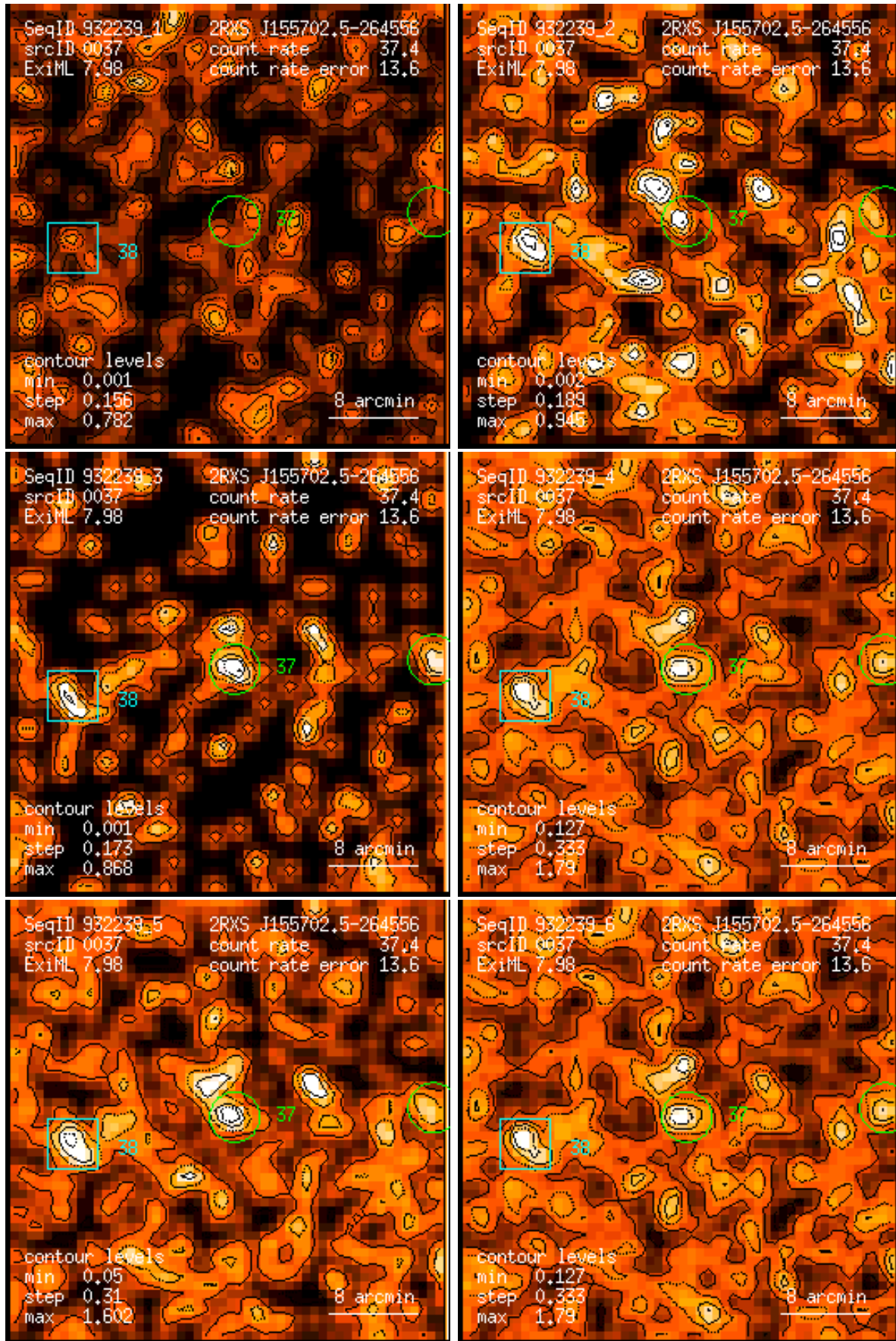
Figure 37: RASS 932239: detection 0037: band rate images, Gaussian filter: (1) PSPC channels 11 – 41, (2) 52 – 90, (3) 91 – 201, (4) 11 – 235, (5) 52 – 201, (6) 11 – 201. Broad band rates in counts/ks. Band rate contour levels in counts/ks/arcmin 2 .
