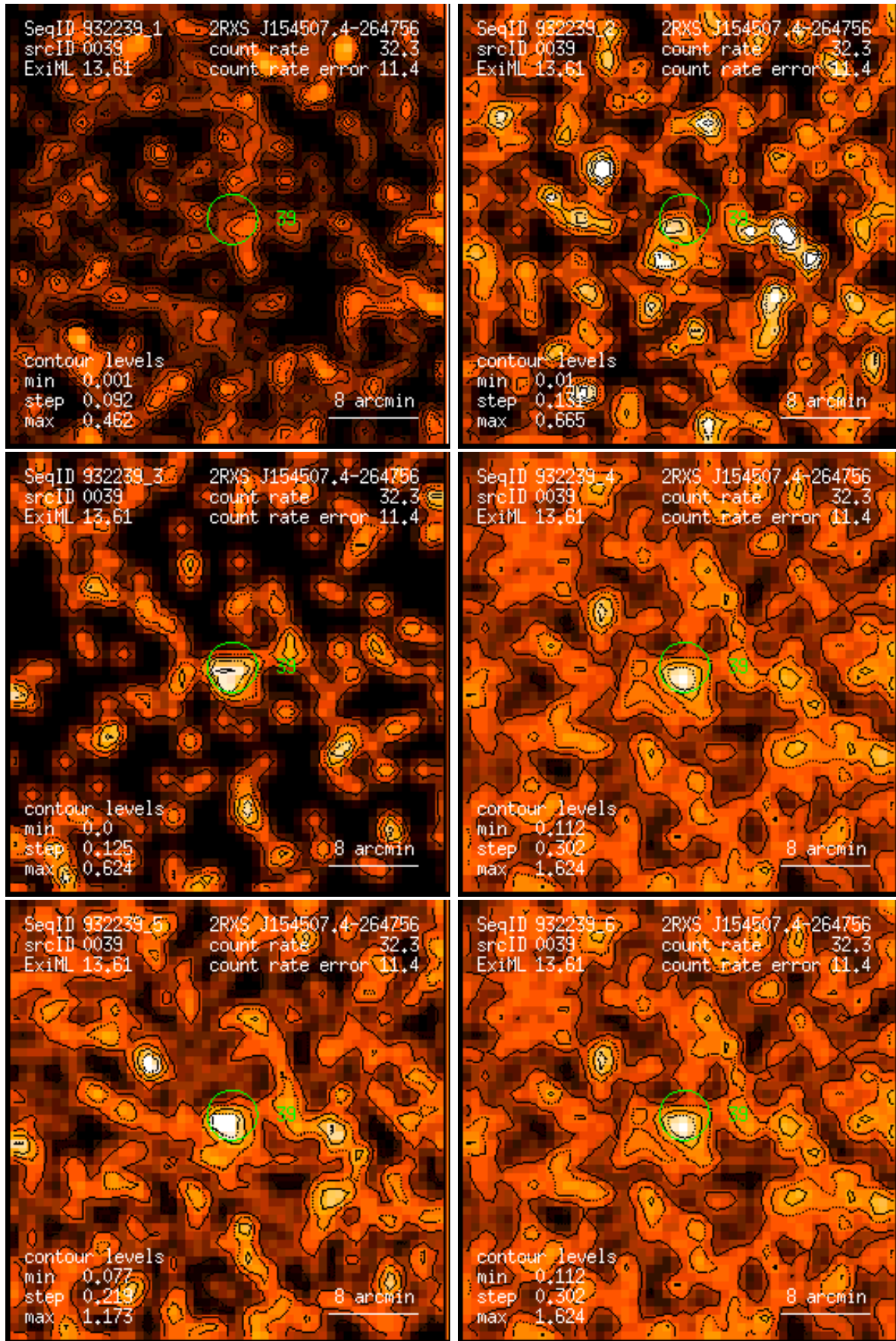
Figure 39: RASS 932239: detection 0039: band rate images, Gaussian filter: (1) PSPC channels 11 – 41, (2) 52 – 90, (3) 91 – 201, (4) 11 – 235, (5) 52 – 201, (6) 11 – 201. Broad band rates in counts/ks. Band rate contour levels in counts/ks/arcmin 2 .
