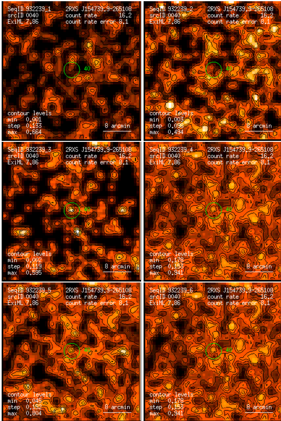
Figure 40: RASS 932239: detection 0040: band rate images, Gaussian filter: (1) PSPC channels 11 – 41, (2) 52 – 90, (3) 91 – 201, (4) 11 – 235, (5) 52 – 201, (6) 11 – 201. Broad band rates in counts/ks. Band rate contour levels in counts/ks/arcmin 2 .
