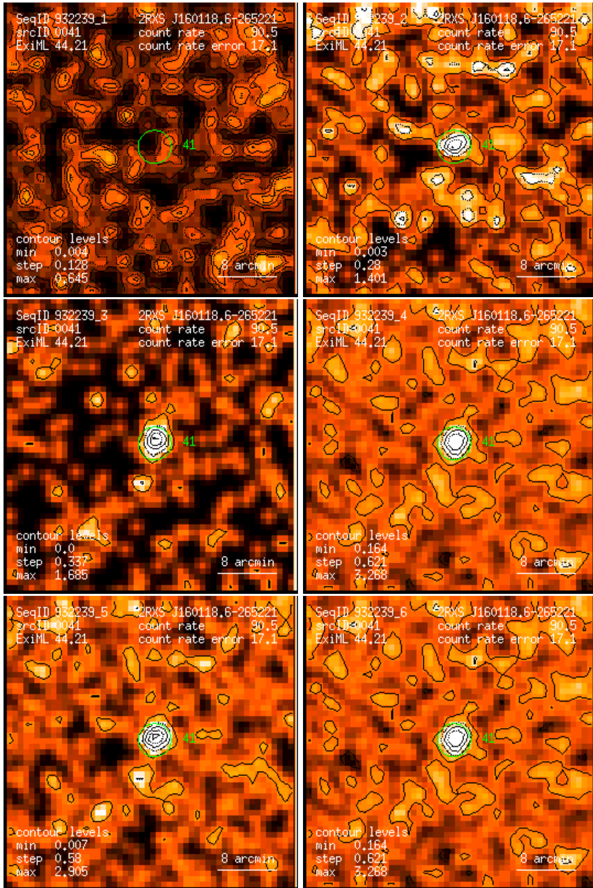
Figure 41: RASS 932239: detection 0041: band rate images, Gaussian filter: (1) PSPC channels 11 – 41, (2) 52 – 90, (3) 91 – 201, (4) 11 – 235, (5) 52 – 201, (6) 11 – 201. Broad band rates in counts/ks. Band rate contour levels in counts/ks/arcmin 2 .
