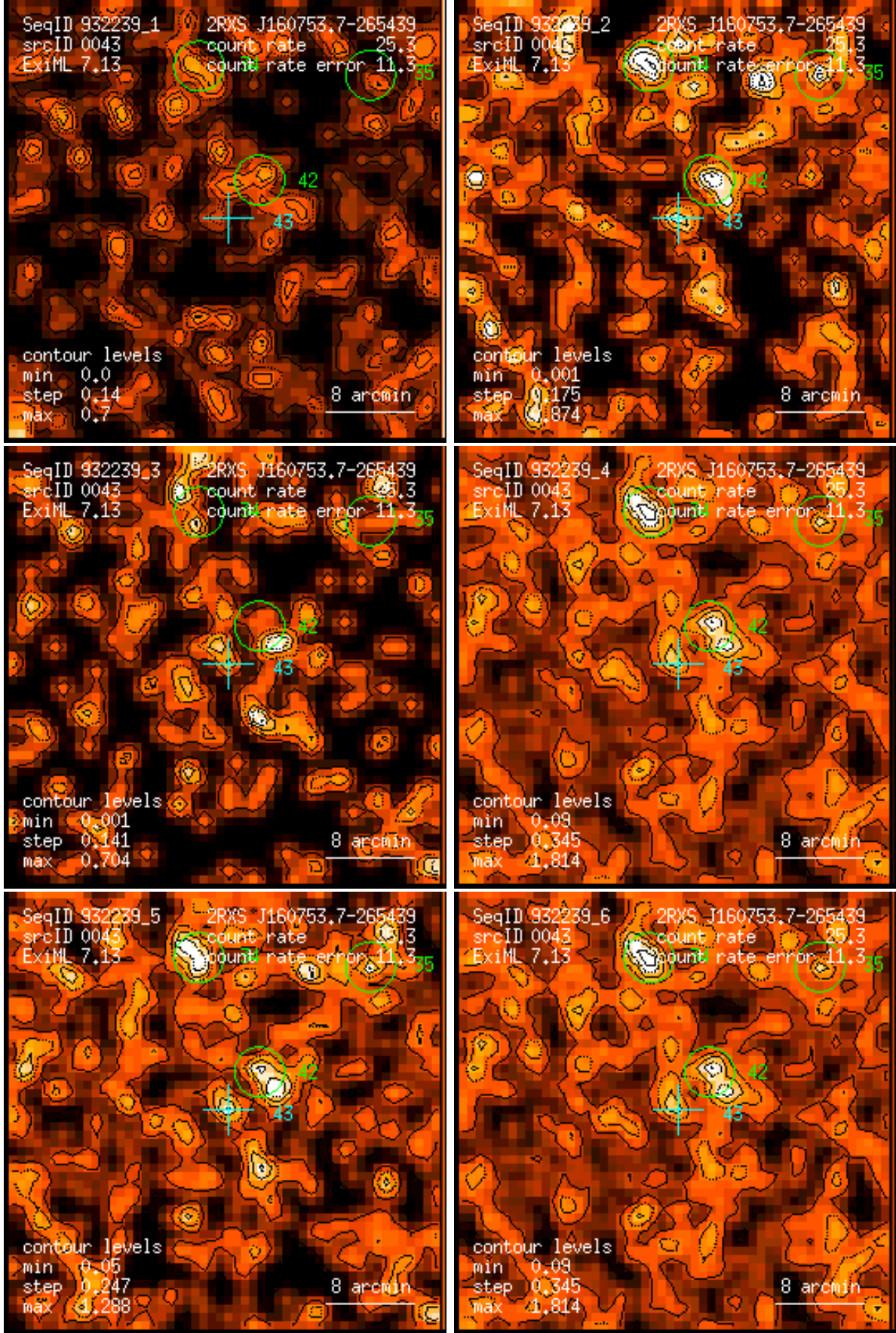
Figure 43: RASS 932239: detection 0043: band rate images, Gaussian filter: (1) PSPC channels 11 – 41, (2) 52 – 90, (3) 91 – 201, (4) 11 – 235, (5) 52 – 201, (6) 11 – 201. Broad band rates in counts/ks. Band rate contour levels in counts/ks/arcmin 2 .
