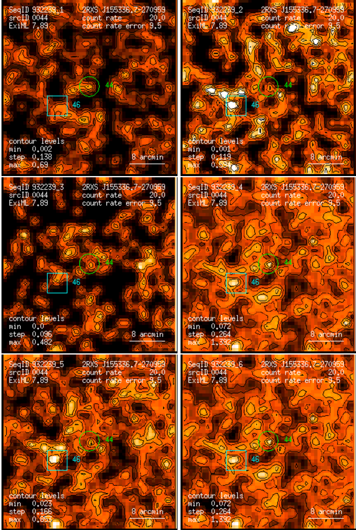
Figure 44: RASS 932239: detection 0044: band rate images, Gaussian filter: (1) PSPC channels 11 – 41, (2) 52 – 90, (3) 91 – 201, (4) 11 – 235, (5) 52 – 201, (6) 11 – 201. Broad band rates in counts/ks. Band rate contour levels in counts/ks/arcmin 2 .
