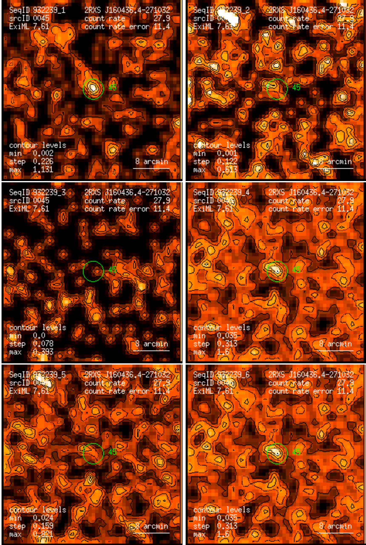
Figure 45: RASS 932239: detection 0045: band rate images, Gaussian filter: (1) PSPC channels 11 – 41, (2) 52 – 90, (3) 91 – 201, (4) 11 – 235, (5) 52 – 201, (6) 11 – 201. Broad band rates in counts/ks. Band rate contour levels in counts/ks/arcmin 2 .
