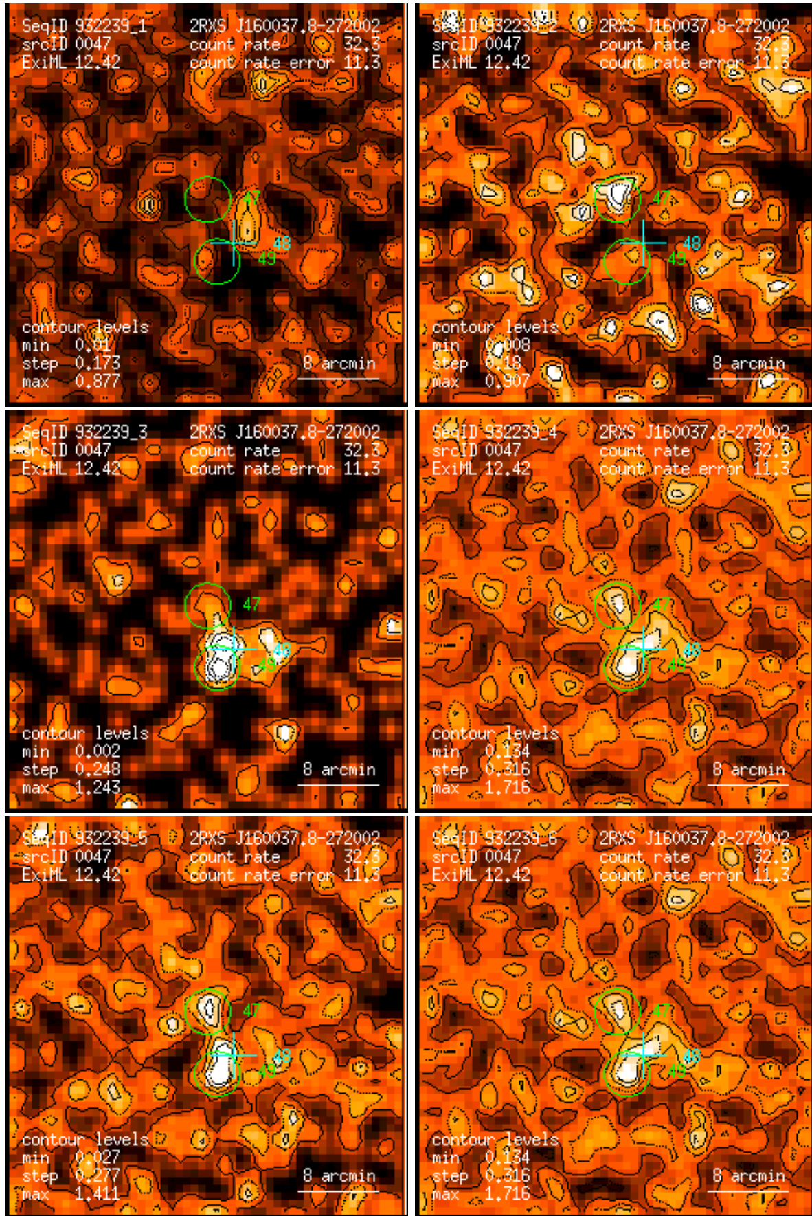
Figure 47: RASS 932239: detection 0047: band rate images, Gaussian filter: (1) PSPC channels 11 – 41, (2) 52 – 90, (3) 91 – 201, (4) 11 – 235, (5) 52 – 201, (6) 11 – 201. Broad band rates in counts/ks. Band rate contour levels in counts/ks/arcmin 2 .
