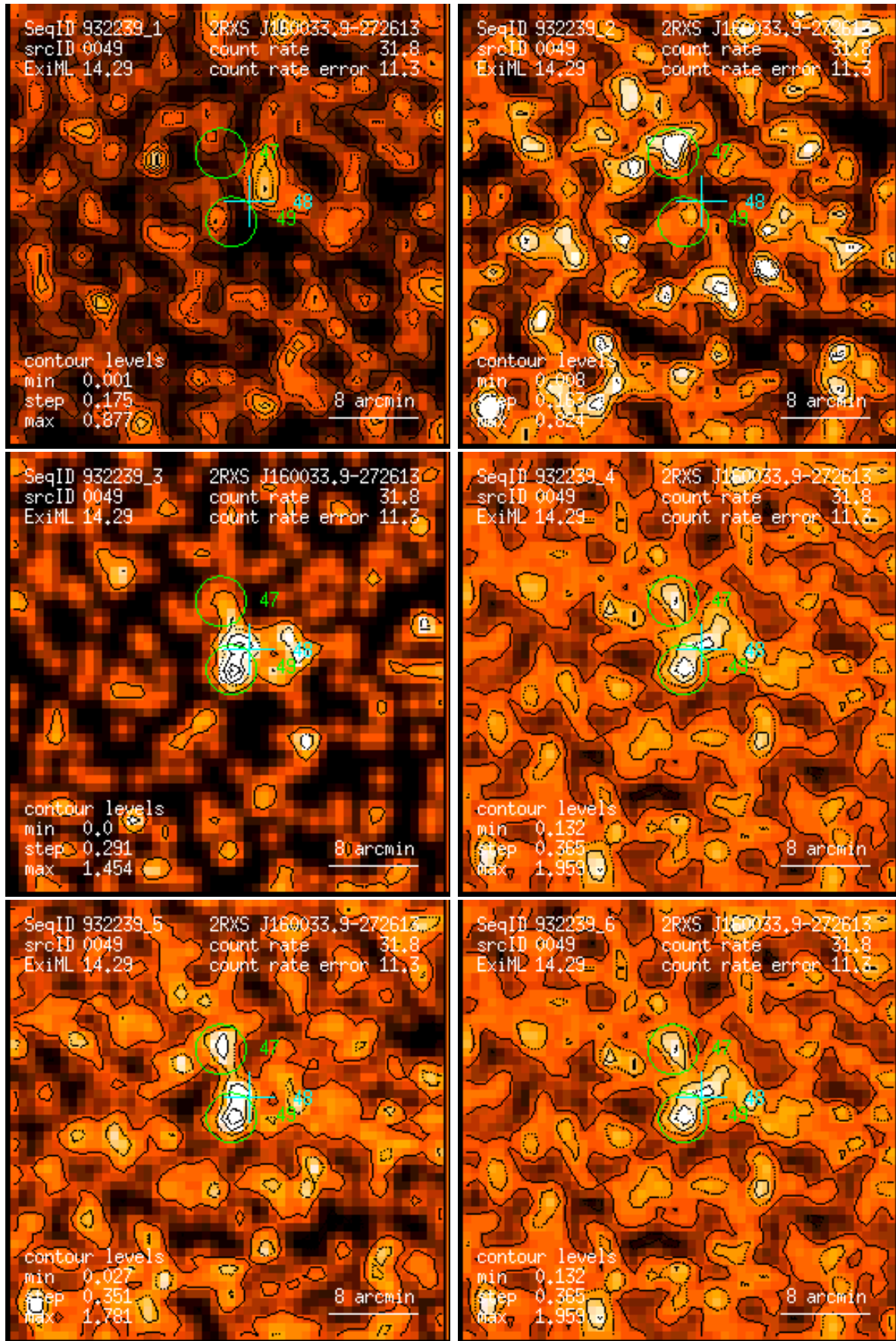
Figure 49: RASS 932239: detection 0049: band rate images, Gaussian filter: (1) PSPC channels 11 – 41, (2) 52 – 90, (3) 91 – 201, (4) 11 – 235, (5) 52 – 201, (6) 11 – 201. Broad band rates in counts/ks. Band rate contour levels in counts/ks/arcmin 2 .
