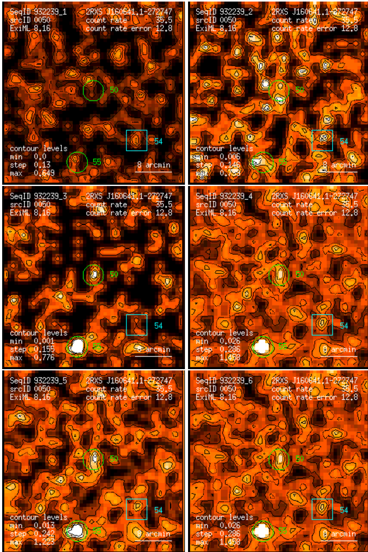
Figure 50: RASS 932239: detection 0050: band rate images, Gaussian filter: (1) PSPC channels 11 – 41, (2) 52 – 90, (3) 91 – 201, (4) 11 – 235, (5) 52 – 201, (6) 11 – 201. Broad band rates in counts/ks. Band rate contour levels in counts/ks/arcmin 2 .
