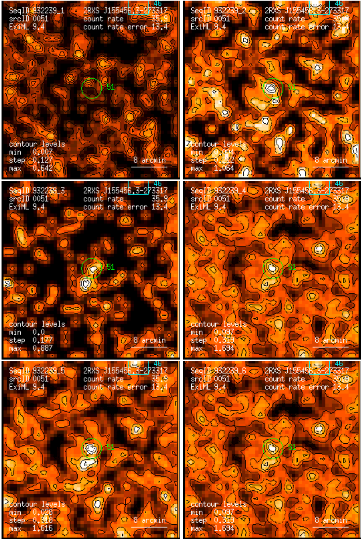
Figure 51: RASS 932239: detection 0051: band rate images, Gaussian filter: (1) PSPC channels 11 – 41, (2) 52 – 90, (3) 91 – 201, (4) 11 – 235, (5) 52 – 201, (6) 11 – 201. Broad band rates in counts/ks. Band rate contour levels in counts/ks/arcmin 2 .
