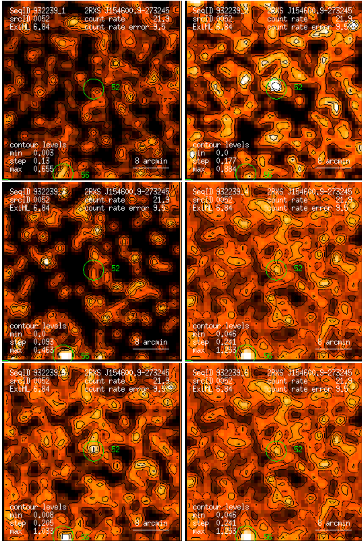
Figure 52: RASS 932239: detection 0052: band rate images, Gaussian filter: (1) PSPC channels 11 – 41, (2) 52 – 90, (3) 91 – 201, (4) 11 – 235, (5) 52 – 201, (6) 11 – 201. Broad band rates in counts/ks. Band rate contour levels in counts/ks/arcmin 2 .
