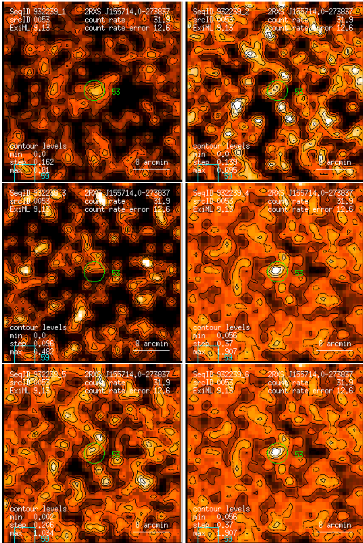
Figure 53: RASS 932239: detection 0053: band rate images, Gaussian filter: (1) PSPC channels 11 – 41, (2) 52 – 90, (3) 91 – 201, (4) 11 – 235, (5) 52 – 201, (6) 11 – 201. Broad band rates in counts/ks. Band rate contour levels in counts/ks/arcmin 2 .
