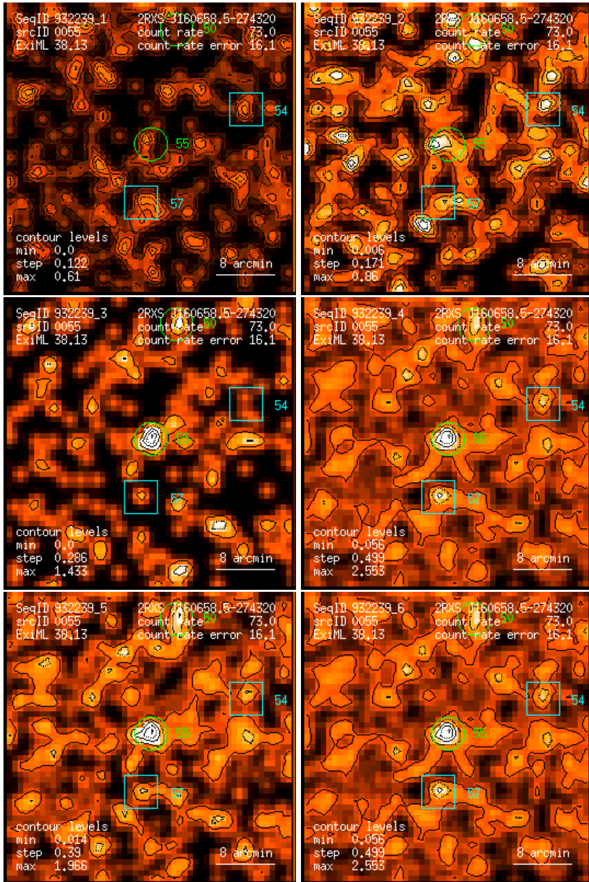
Figure 55: RASS 932239: detection 0055: band rate images, Gaussian filter: (1) PSPC channels 11 – 41, (2) 52 – 90, (3) 91 – 201, (4) 11 – 235, (5) 52 – 201, (6) 11 – 201. Broad band rates in counts/ks. Band rate contour levels in counts/ks/arcmin 2 .
