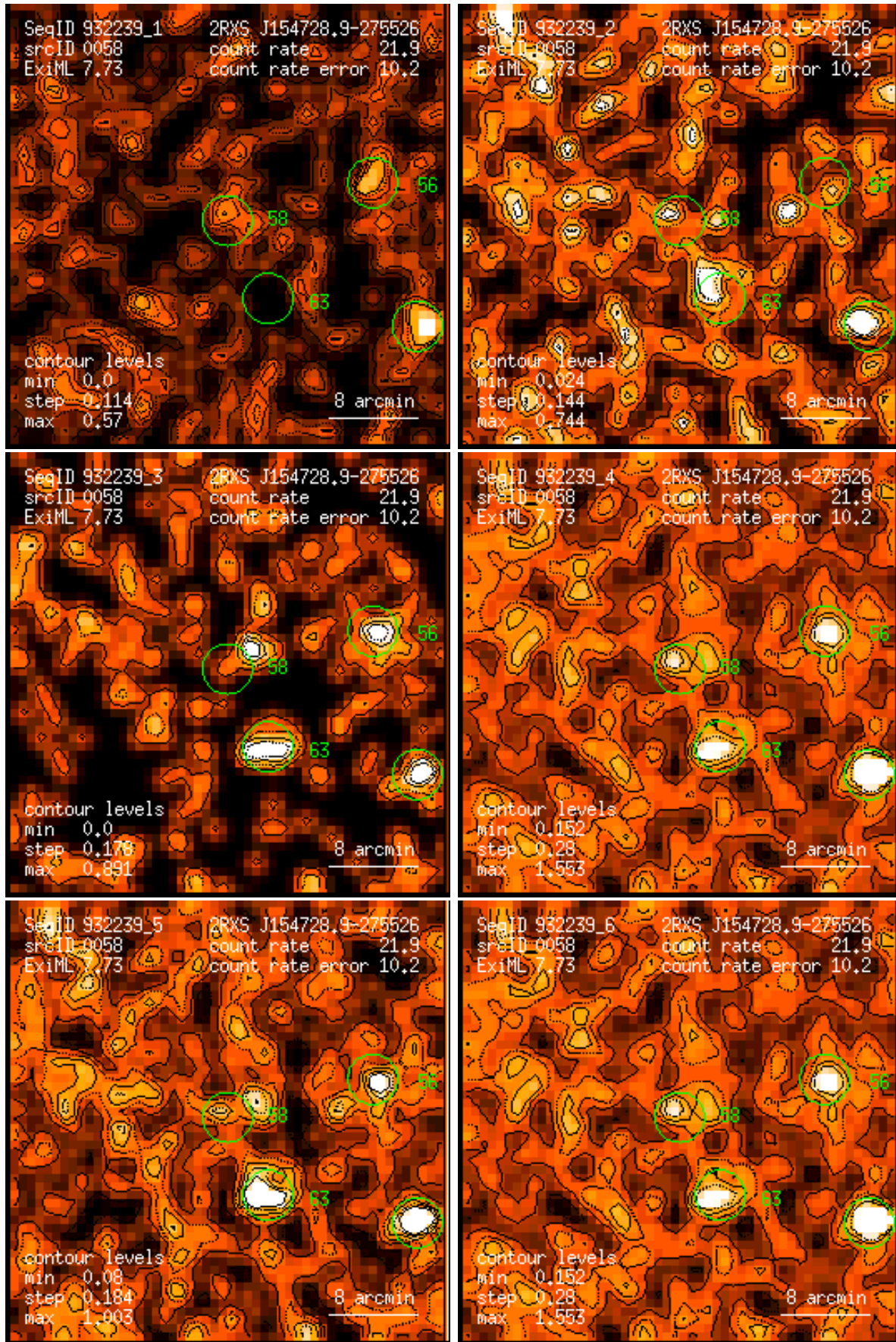
Figure 58: RASS 932239: detection 0058: band rate images, Gaussian filter: (1) PSPC channels 11 – 41, (2) 52 – 90, (3) 91 – 201, (4) 11 – 235, (5) 52 – 201, (6) 11 – 201. Broad band rates in counts/ks. Band rate contour levels in counts/ks/arcmin 2 .
