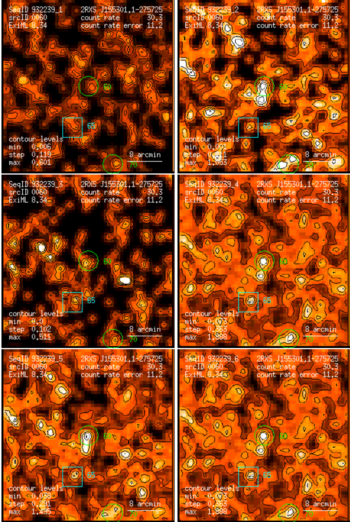
Figure 60: RASS 932239: detection 0060: band rate images, Gaussian filter: (1) PSPC channels 11 – 41, (2) 52 – 90, (3) 91 – 201, (4) 11 – 235, (5) 52 – 201, (6) 11 – 201. Broad band rates in counts/ks. Band rate contour levels in counts/ks/arcmin 2 .
