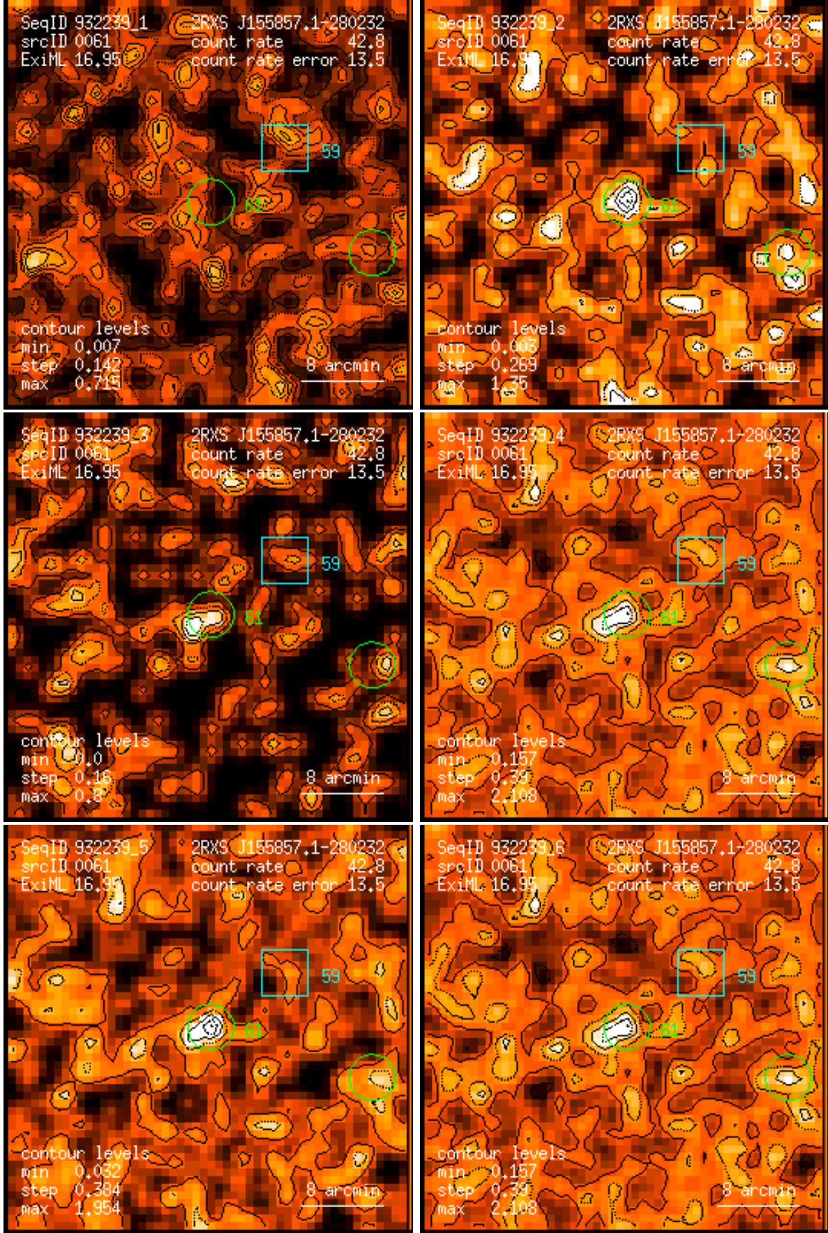
Figure 61: RASS 932239: detection 0061: band rate images, Gaussian filter: (1) PSPC channels 11 – 41, (2) 52 – 90, (3) 91 – 201, (4) 11 – 235, (5) 52 – 201, (6) 11 – 201. Broad band rates in counts/ks. Band rate contour levels in counts/ks/arcmin 2 .
