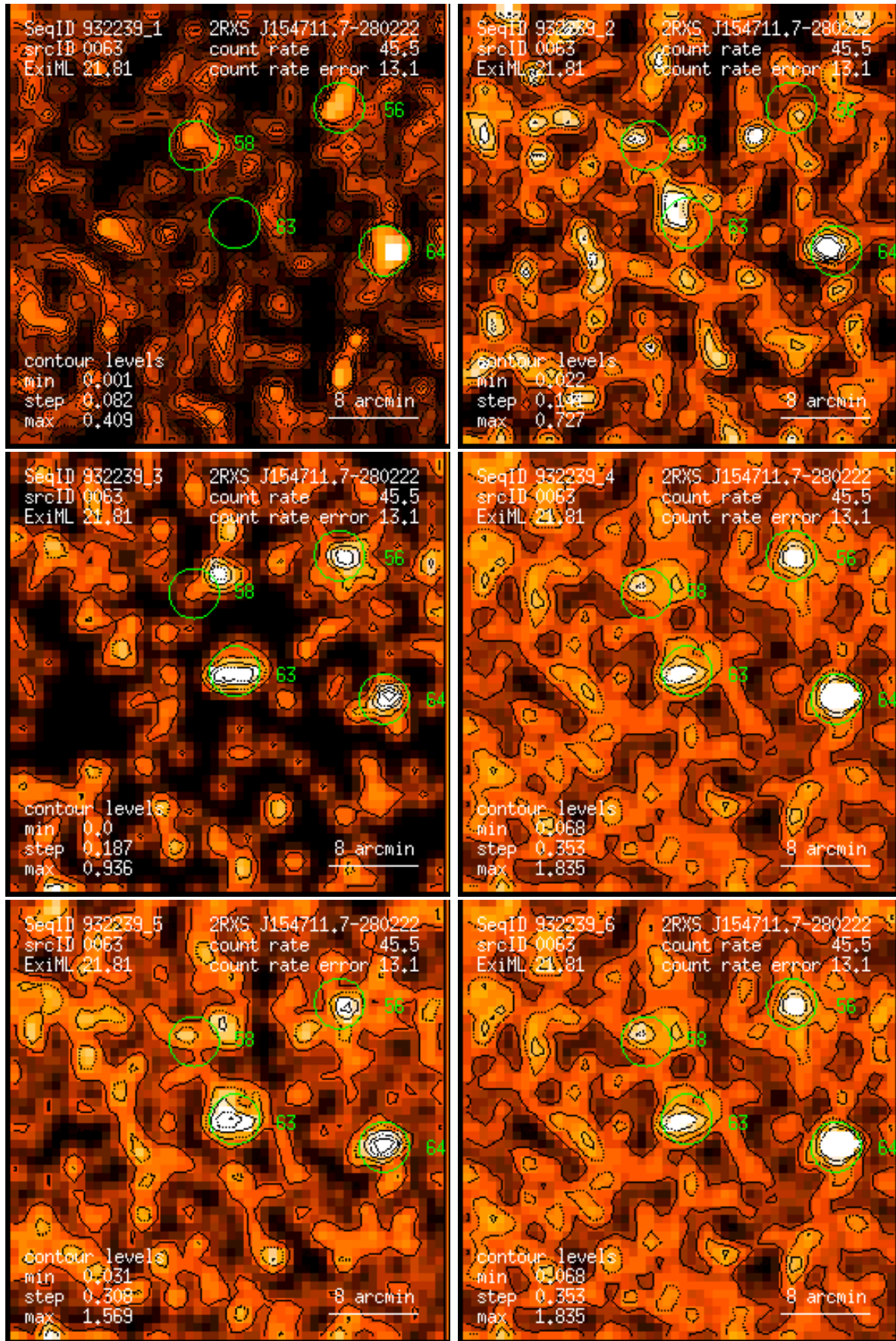
Figure 63: RASS 932239: detection 0063: band rate images, Gaussian filter: (1) PSPC channels 11 – 41, (2) 52 – 90, (3) 91 – 201, (4) 11 – 235, (5) 52 – 201, (6) 11 – 201. Broad band rates in counts/ks. Band rate contour levels in counts/ks/arcmin 2 .
