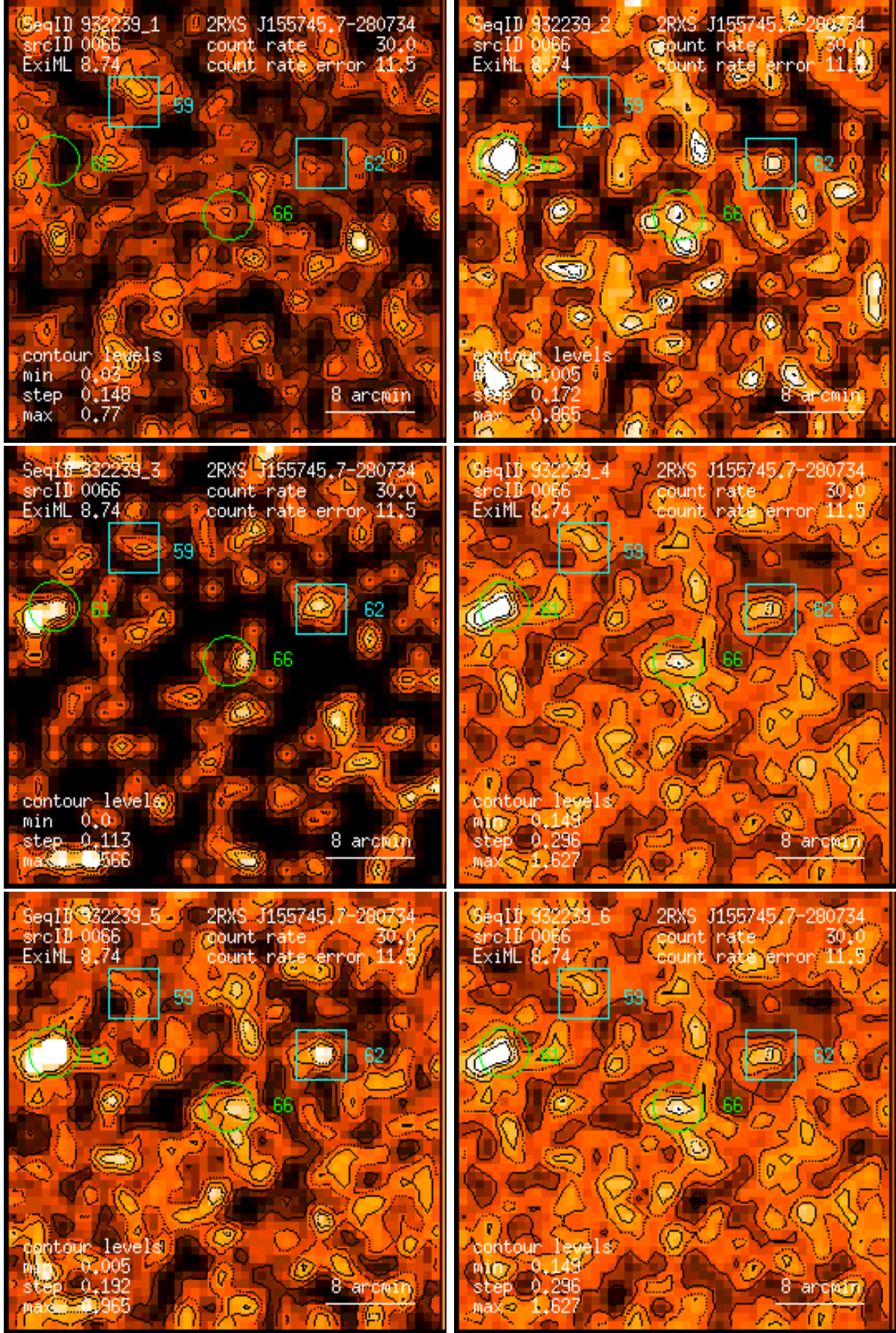
Figure 66: RASS 932239: detection 0066: band rate images, Gaussian filter: (1) PSPC channels 11 – 41, (2) 52 – 90, (3) 91 – 201, (4) 11 – 235, (5) 52 – 201, (6) 11 – 201. Broad band rates in counts/ks. Band rate contour levels in counts/ks/arcmin 2 .
