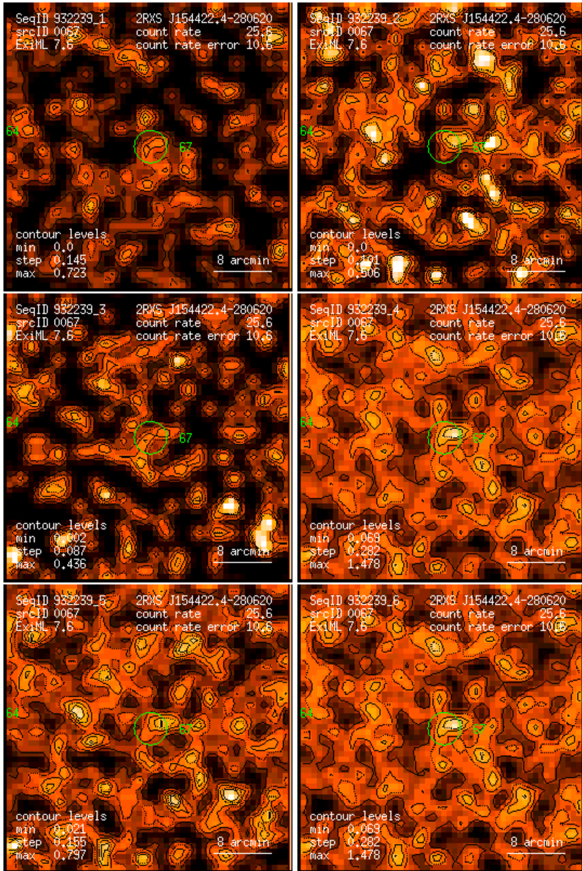
Figure 67: RASS 932239: detection 0067: band rate images, Gaussian filter: (1) PSPC channels 11 – 41, (2) 52 – 90, (3) 91 – 201, (4) 11 – 235, (5) 52 – 201, (6) 11 – 201. Broad band rates in counts/ks. Band rate contour levels in counts/ks/arcmin 2 .
