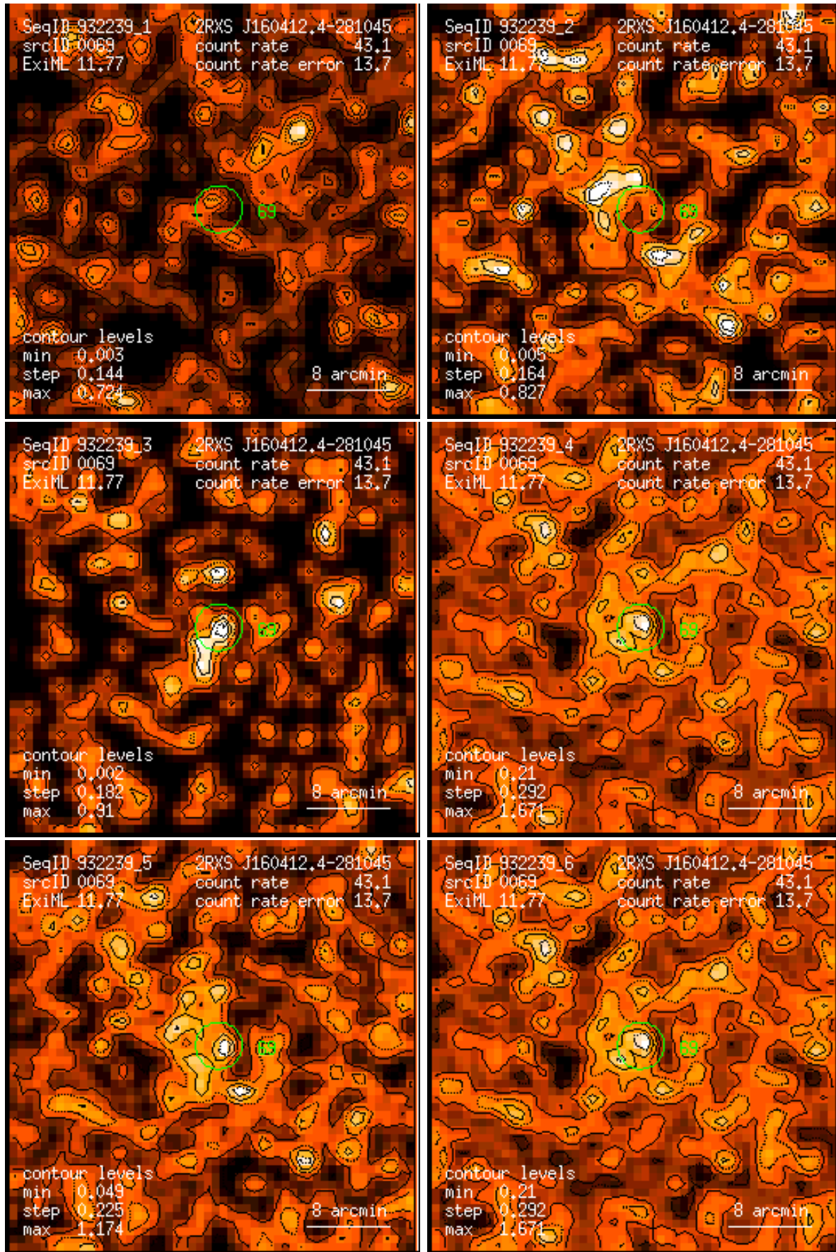
Figure 69: RASS 932239: detection 0069: band rate images, Gaussian filter: (1) PSPC channels 11 – 41, (2) 52 – 90, (3) 91 – 201, (4) 11 – 235, (5) 52 – 201, (6) 11 – 201. Broad band rates in counts/ks. Band rate contour levels in counts/ks/arcmin 2 .
