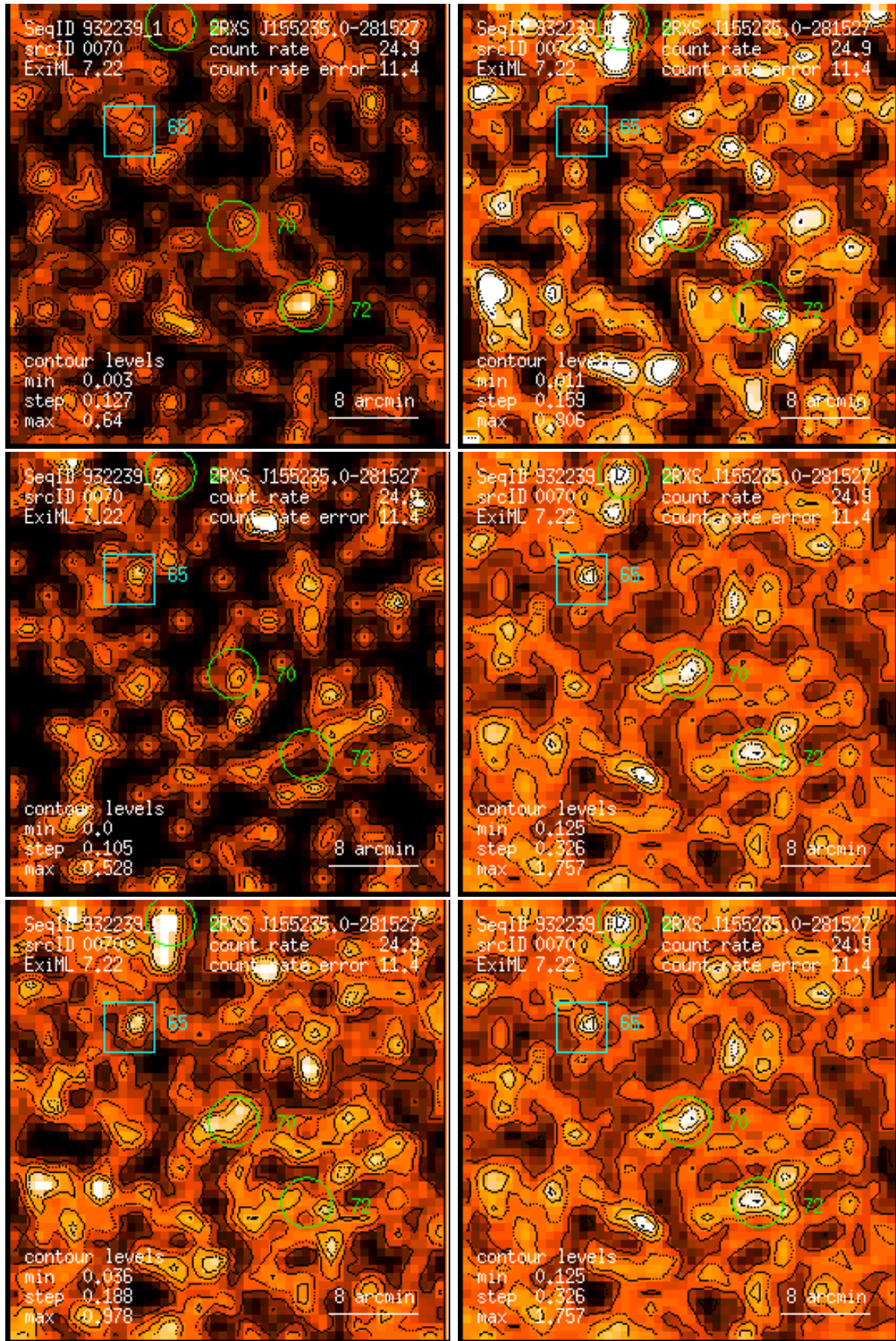
Figure 70: RASS 932239: detection 0070: band rate images, Gaussian filter: (1) PSPC channels 11 – 41, (2) 52 – 90, (3) 91 – 201, (4) 11 – 235, (5) 52 – 201, (6) 11 – 201. Broad band rates in counts/ks. Band rate contour levels in counts/ks/arcmin 2 .
